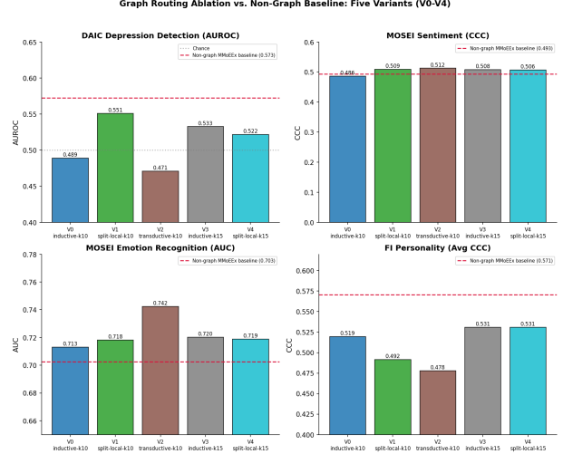
Figure 6: Graph routing ablation vs. the non-graph MMoEEx baseline (red dashed line), all five variants across the 5-seed protocol.
