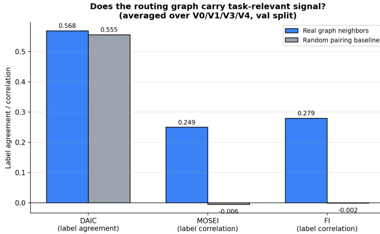
Figure 1.5: Real graph neighbors vs. random pairing, averaged over V0/V1/V3/V4 (val split). DAIC shows no signal beyond chance; MOSEI and FI both show substantial signal that the router fails to exploit.
