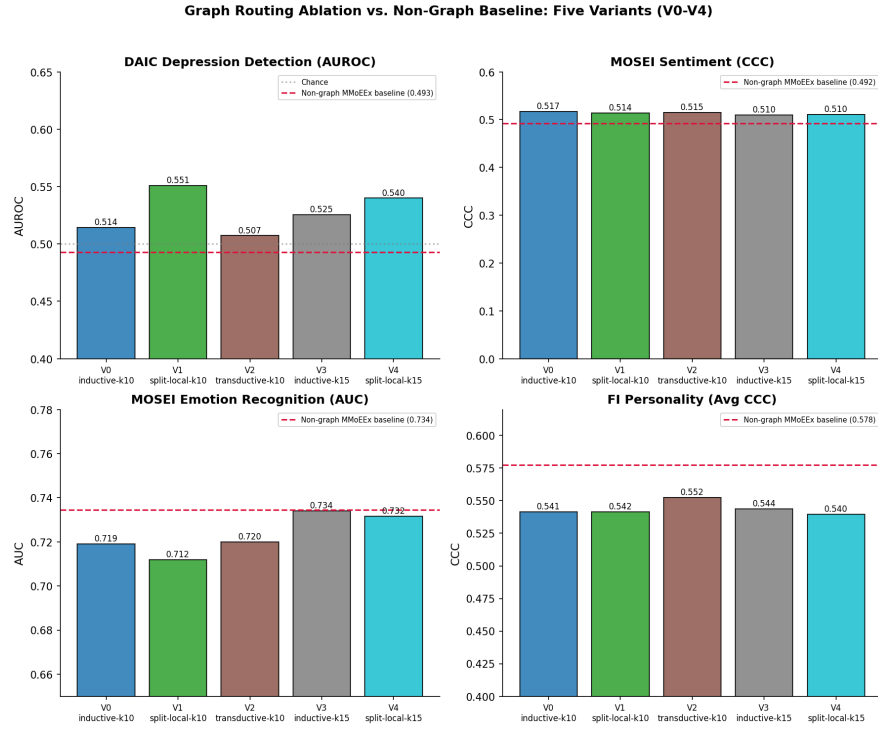
Figure 1.4: Graph routing ablation vs. the non-graph MMoEEx baseline (red dashed line), five variants (V0–V4). Graph routing gives a small, inconsistent edge on DAIC AUROC, roughly ties MOSEI, and is consistently below the baseline on FI personality.
