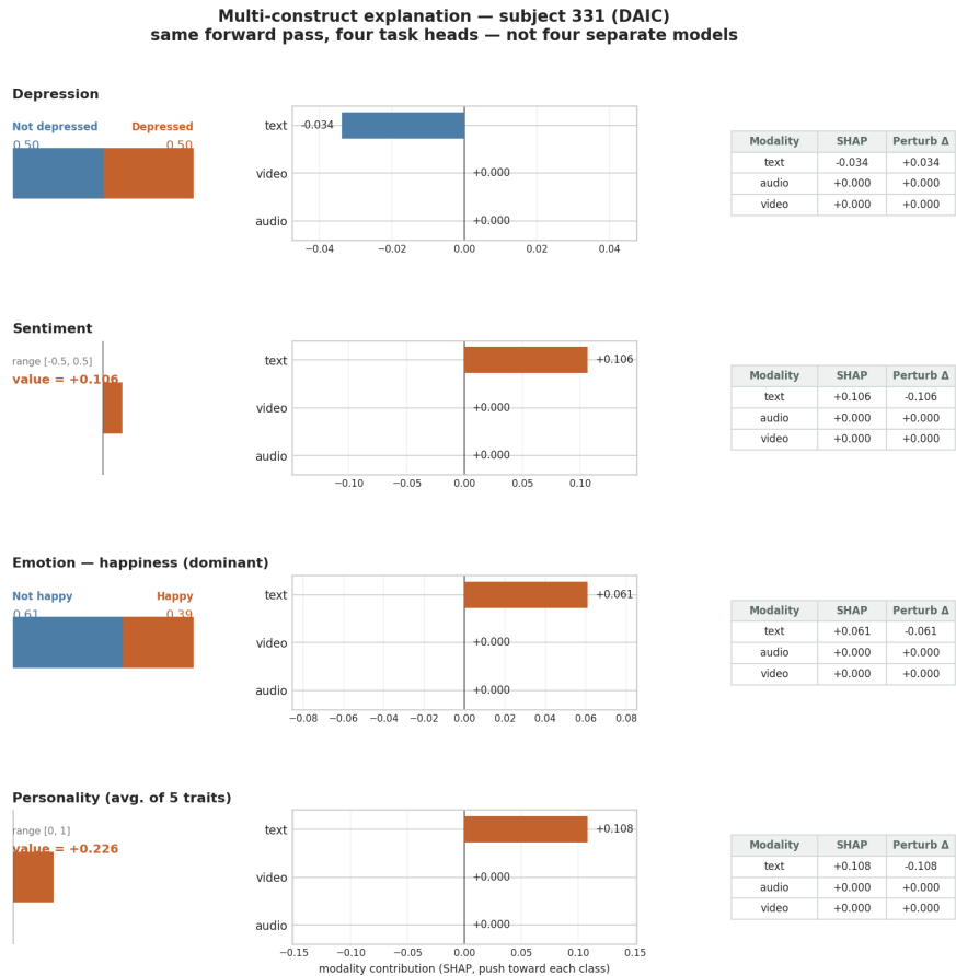
Figure 1.13: Multi-construct force plot: one DAIC subject’s shared representation, explained through all four task heads in a single figure (prediction bar, per-modality SHAP tornado, and value table per row) rather than as four disconnected numbers. Audio and video read exactly zero on every row, directly visualizing the text-only routing policy rather than leaving it implicit in a table. See per-dataset versions in artifacts/figures/phase_11_xai/ .
