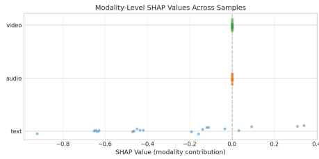
Figure 1.11: SHAP beeswarm plot for DAIC: modality-level contributions across 20 real samples from the validation set. Audio and video collapse to exactly zero for every sample, since DAIC is evaluated under text-only routing (Section 1.6.2) and its fused representation structurally excludes them; only text shows any spread. See artifacts/figures/phase_11_xai/ for per-dataset versions.
