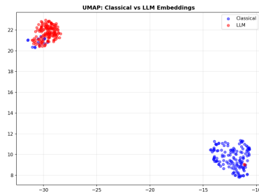
Figure 1.10: UMAP comparison of classical (RoBERTa, 768D, blue) vs LLM (Mistral-7B, 4096D, red) text embeddings for 154 samples across DAIC, MOSEI, and FI. Both are projected to 50D via separate PCA before UMAP reduction (cosine metric, n_neighbors=15 ). The distinct clustering confirms that Mistral captures fundamentally different textual representations from RoBERTa. Source: artifacts/figures/phase_08_llm_ablations/embedding_umap.png .
