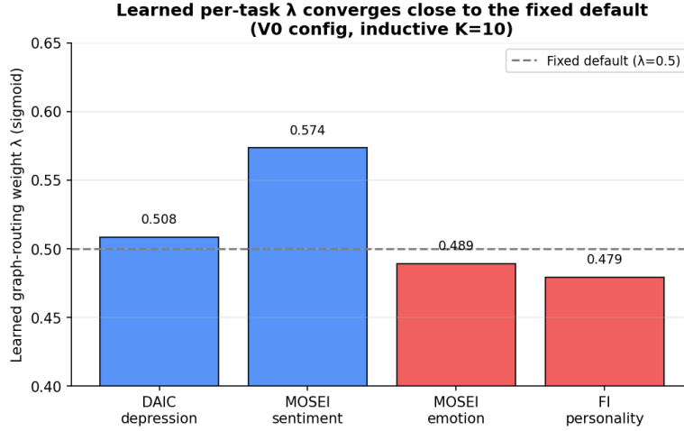
Figure 1.7: Learned per-task \lambda (V0 configuration) moves in the direction the homophily diagnostic predicts, but only slightly.
