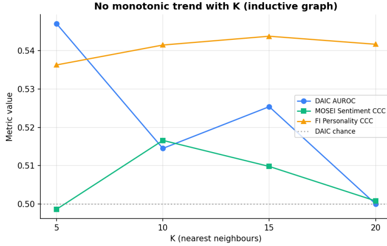
Figure 1.6: No monotonic trend with K (inductive graph, DAIC/MOSEI/FI).
