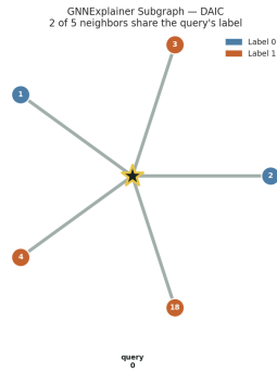
Figure 1.12: Ego-centered subgraph for a DAIC query sample (star, center). Neighbors sit at a radius proportional to their dissimilarity in the model’s trained fused representation and are colored by their true depression label, so label agreement is visible directly: here 2 of 5 neighbors share the query’s label, consistent with the below-random homophily finding (Section 1.6.4). See per-dataset versions in artifacts/figures/phase_11_xai/ .
