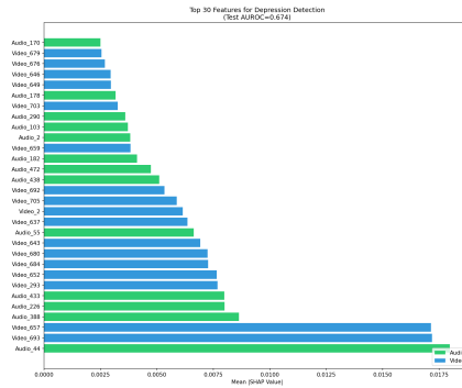
Figure 1.8: Top 30 features by SHAP importance for MPDD-Young depression detection. Audio features are shown in green, video features in blue. The single most important feature is audio_44 (SHAP=0.018), followed by video_693 and video_657.
