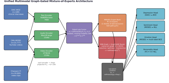
Figure 1: Unified multimodal graph-gated MoE architecture.
