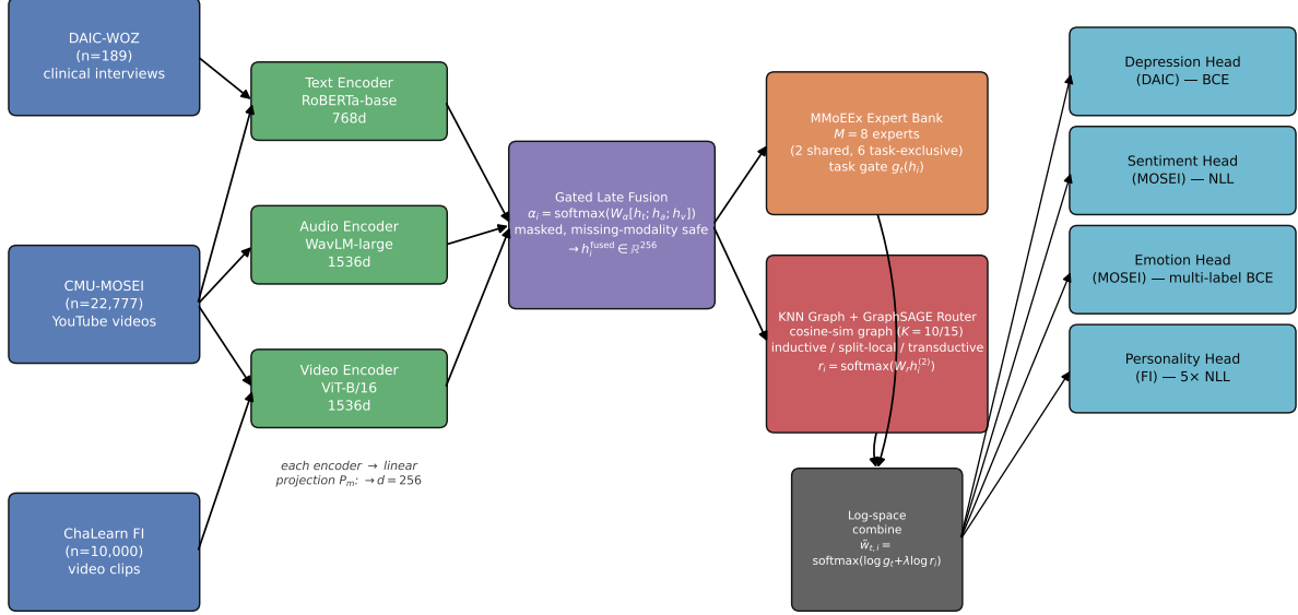
Unified Multimodal Graph-Gated Mixture-of-Experts Architecture
