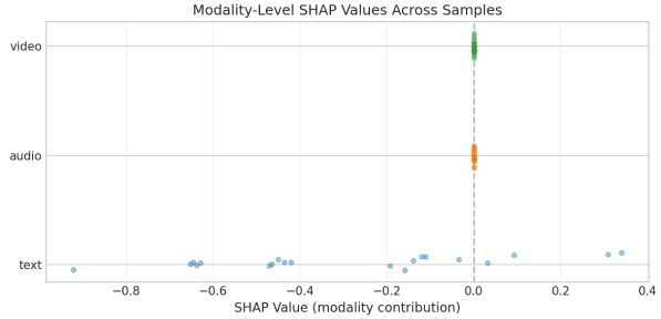
Figure 13: Per-modality SHAP values across 20 DAIC validation samples. Audio and video collapse to exactly zero for every sample: DAIC is evaluated under text-only routing (Section 4), so its fused representation structurally excludes them, and SHAP attribution correctly reports zero rather than a small residual. Only text shows any spread.
