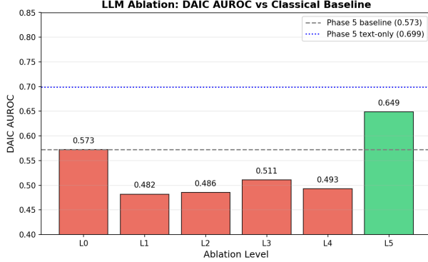
Figure 10: LLM modality ablation: DAIC AUROC per level (L0–L5) against the classical (L0) and Phase-5 text-only baselines.
