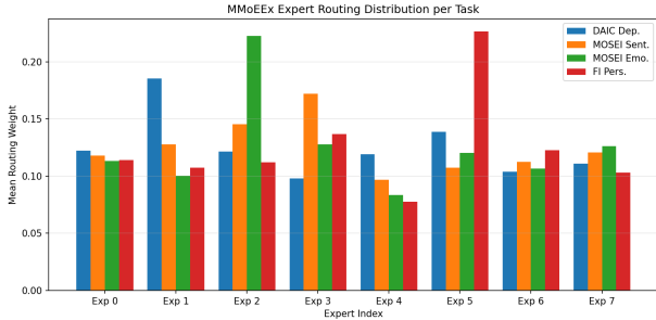
Figure 5: Mean MMoEE expert routing weight per expert and task. Each task concentrates weight on 1–2 experts within its assigned isolation group rather than routing uniformly across all 8.
