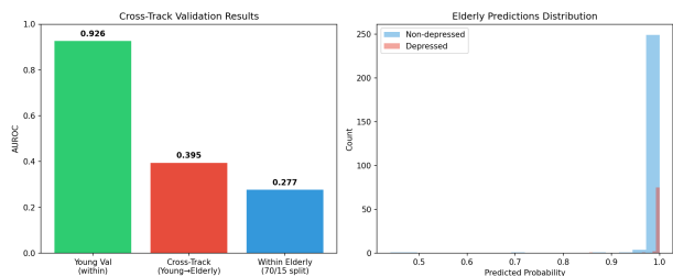
Figure 12: Left: AUROC within Young, cross-track Young→Elderly, and within Elderly. Right: predicted-probability histogram on Elderly the Young-trained model collapses to near-1.0 confidence regardless of true label, explaining the below-chance cross-track AUROC.
