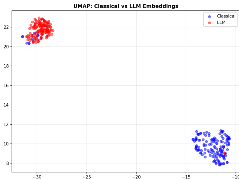
Figure 1.5: UMAP comparison of classical (RoBERTa, 768D, blue) vs LLM (Mistral-7B, 4096D, red) text embeddings for 154 samples across DAIC, MOSEI, and FI. Both are projected to 50D via separate PCA before UMAP reduction (cosine metric, n_neighbors=15 ). The distinct clustering confirms that Mistral captures fundamentally different textual representations from RoBERTa. Source: artifacts/figures/phase_08_llm_ablations/embedding_umap.png .
