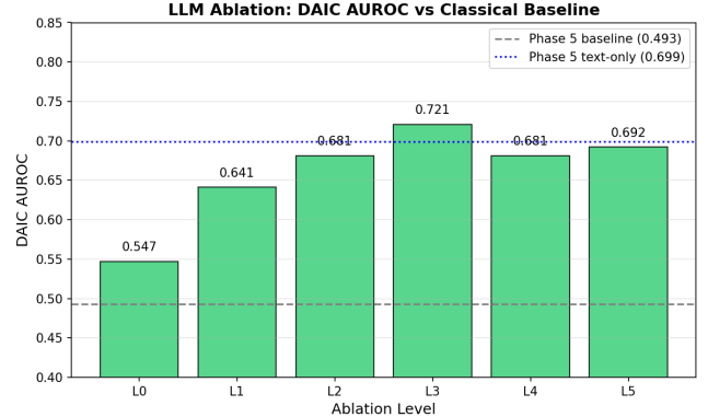
Figure 4: LLM modality ablation: DAIC AUROC per level (L0–L5) against the classical (L0) and Phase-5 text-only baselines. L3 (Mistral+CLAP) gives the largest gain.
