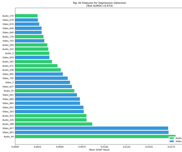
Figure 5: Top-30 SHAP feature importances for MPDD-Young depression detection. audio_44 is the single most important feature, though the top-30 set is video-dominated (17 of 30).
