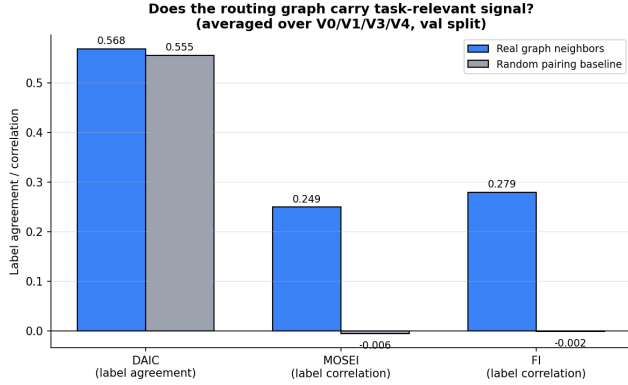
Figure 3: Real graph neighbours vs. random pairing, averaged over V0/V1/V3/V4. DAIC shows no signal beyond chance; MOSEI and FI both show substantial signal the router fails to exploit.
