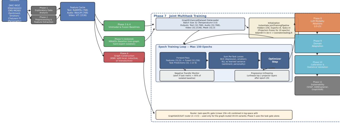
Figure 2: Implementation detail of joint multitask training (Phase 7) and the non-graph MMoEEx baseline that precedes it (Phase 5): DataLoader tensor shapes, initialization, the epoch loop, and the negative-transfer monitor and progressive-unfreezing mechanisms. The graph router (bottom right) applies only to the graph-routed V0–V4 variants shown in Figure 1; Phase 5 uses the task gate alone.
