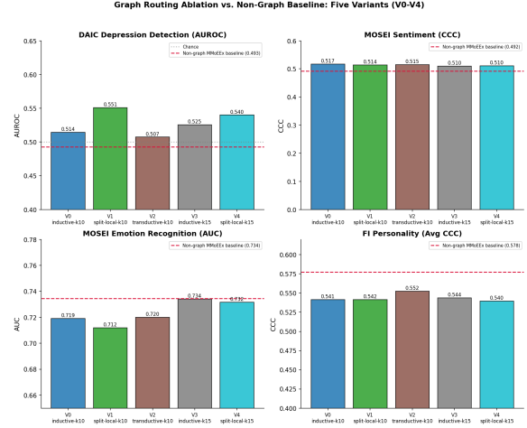
Figure 5: Graph routing ablation vs. non-graph MMoEEx baseline (red dashed line), all five variants across all four tasks.
