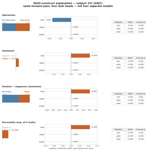
Figure 9: Multi-construct force plot: one DAIC subject explained through all four task heads in a single figure. Audio and video read exactly zero on every row, visualizing DAIC’s text-only routing directly rather than leaving it implicit.
