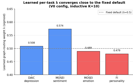
Figure 4: Learned per-task \lambda (V0 configuration) vs. the fixed default (0.5). Moves down for FI/MOSEI-emotion and up for MOSEI-sentiment/DAIC, consistent with the homophily diagnostic (main paper, Table 2), but only slightly.
