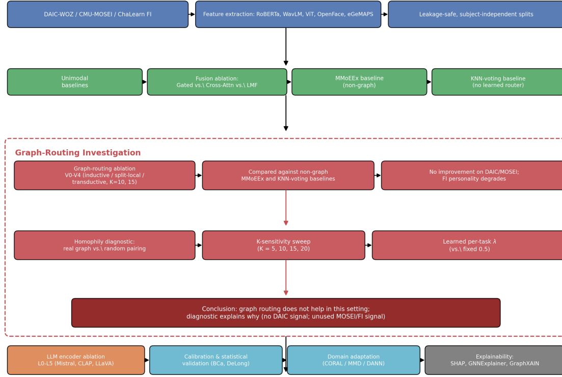
Figure 1: Experimental pipeline overview. The graph-routing investigation (dashed box) is the central empirical question of the main paper: five ablation variants are compared against non-graph baselines, and a homophily diagnostic together with two targeted fixes (K-sweep, learned \lambda ) explains the resulting negative finding.
