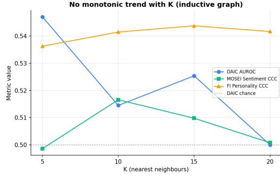
Figure 3: No monotonic trend with K \in \{5, 10, 15, 20\} (inductive graph). K=20 lands DAIC AUROC exactly at chance (0.500).
