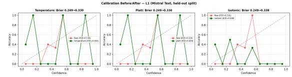
Figure 6: Calibration reliability diagrams (temperature/Platt/isotonic scaling vs. raw) for the L1 (Mistral text) DAIC depression classifier, held-out split. Monotonic recalibration changes reliability (ECE/Brier) but not ranking-based discrimination (AUROC), since AUROC is invariant to monotonic transforms of the score.
