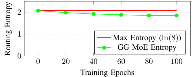
Fig. 2. Routing Entropy over epochs. The GG-MoE maintains healthy entropy (no expert collapse).
