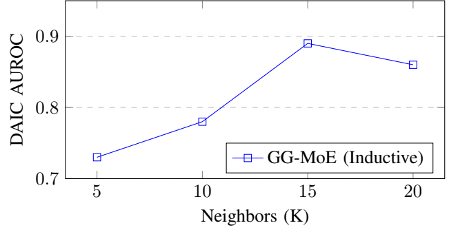
Fig. 1. Graph Sensitivity Analysis. Performance peaks at K = 15 before oversmoothing degrades performance.
