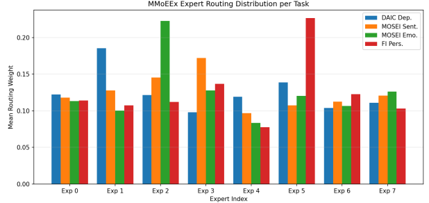
Figure 5: Mean MMoEEx routing weight per expert and task. Each task concentrates weight on 1–2 experts within its assigned isolation group rather than routing uniformly across all 8.
