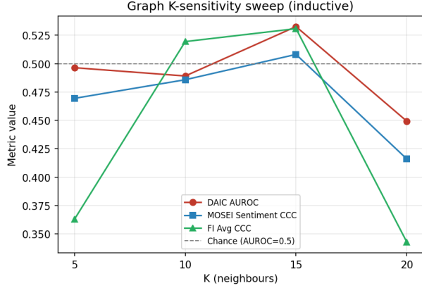
Figure 8: 5-seed mean \pm std, inductive graph: no monotonic trend with K , and no configuration’s DAIC delta from the non-graph baseline is reportable under SPEC-H4-03.
