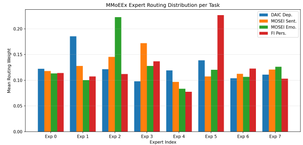
Figure 6: Mean MMoEEEx routing weight per expert and task. Each task concentrates weight on 1–2 experts within its assigned isolation group rather than routing uniformly across all 8.
