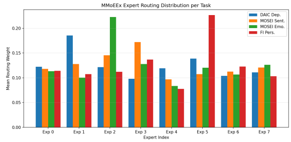
Figure 7: Mean MMoEEx routing weight per expert and task (non-graph baseline). Rows/legend are tasks; columns are the 8 experts.
