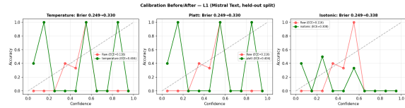
Figure 6: Calibration reliability diagrams (temperature/Platt/isotonic scaling vs. raw) for the L1 (Mistral text) DAIC depression classifier, held-out split. Monotonic recalibration changes reliability (ECE/Brier) but not ranking-based discrimination (AUROC), since AUROC is invariant to monotonic transforms of the score.
