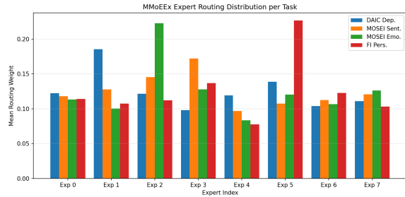
Figure 5: Mean MMEEx routing weight per expert and task (non-graph baseline). Rows/legend are tasks; columns are the 8 experts.
