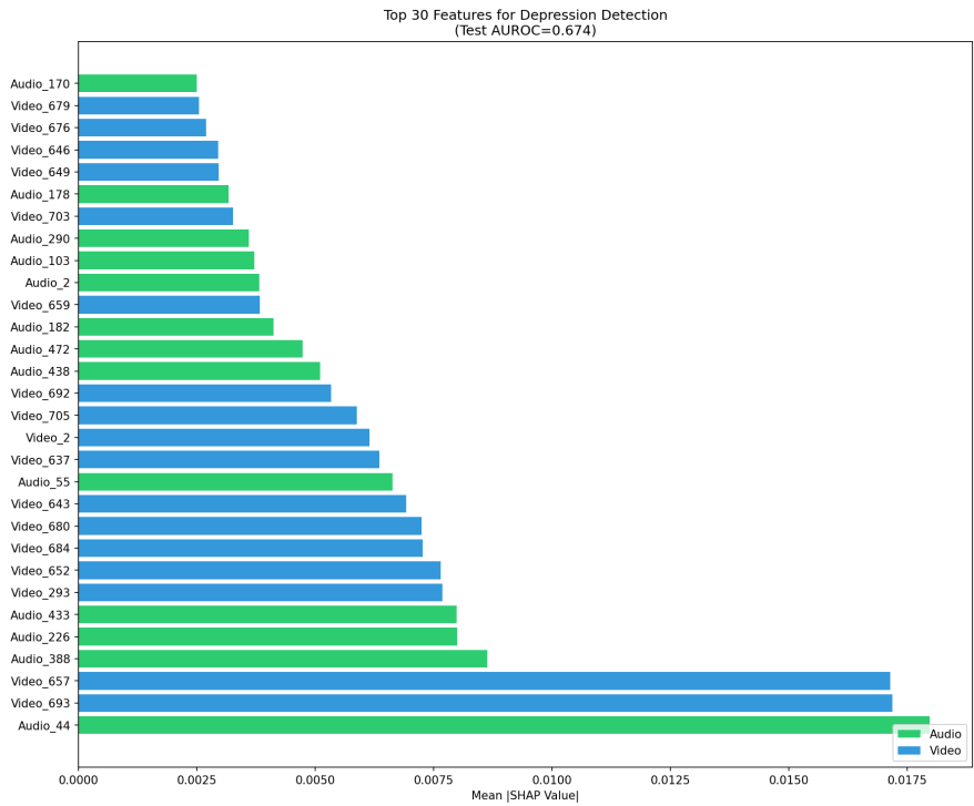
Figure 1.4: Top 30 features by SHAP importance for MPDD-Young depression detection. Audio features are shown in green, video features in blue. The single most important feature is audio_44 (SHAP=0.018), followed by video_693 and video_657 .
