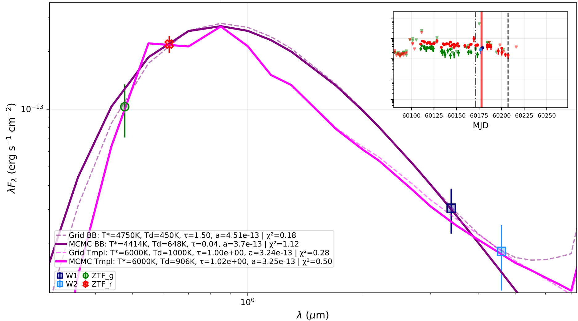
ZTF23aanymcl: SED at MJD 60177.76 (Phase 69.9 d)
