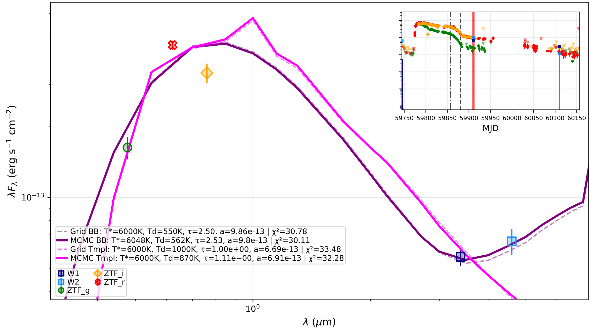
ZTF22aativsd: SED at MJD 59910.55 (Phase 137.1 d)
