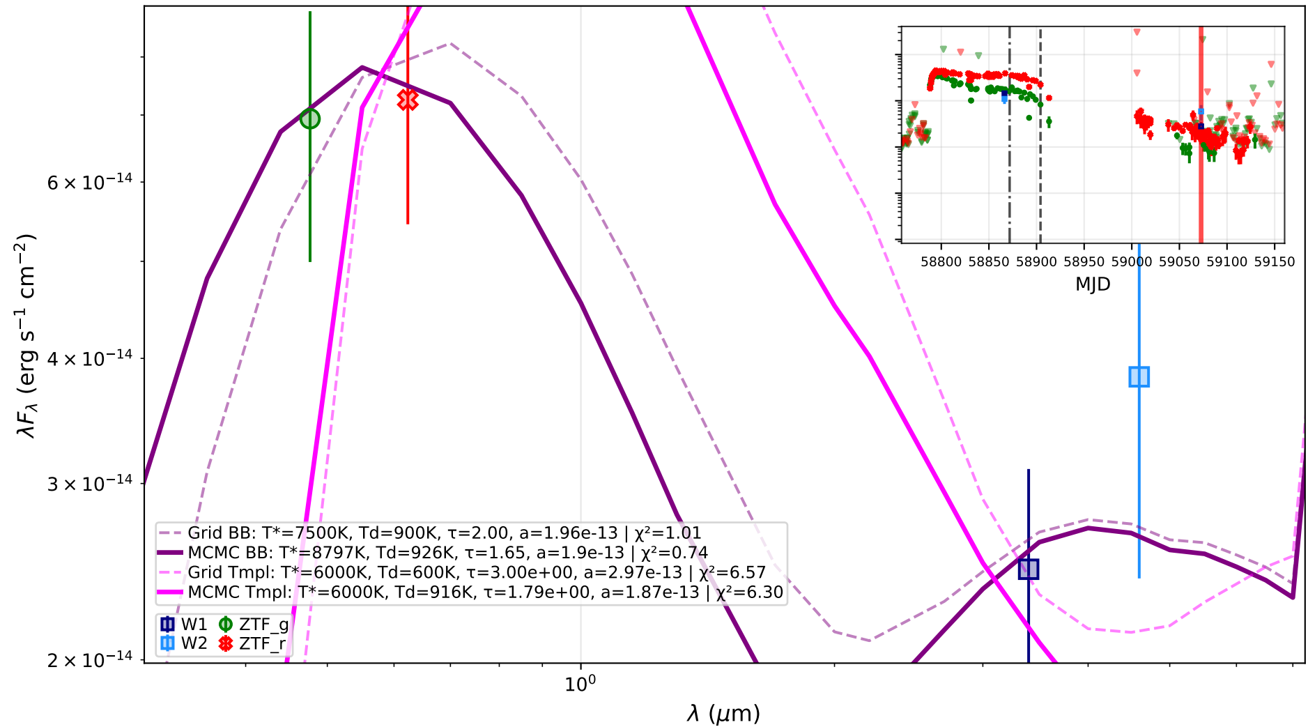
ZTF19aclobbu: SED at MJD 59072.79 (Phase 285.5 d)
