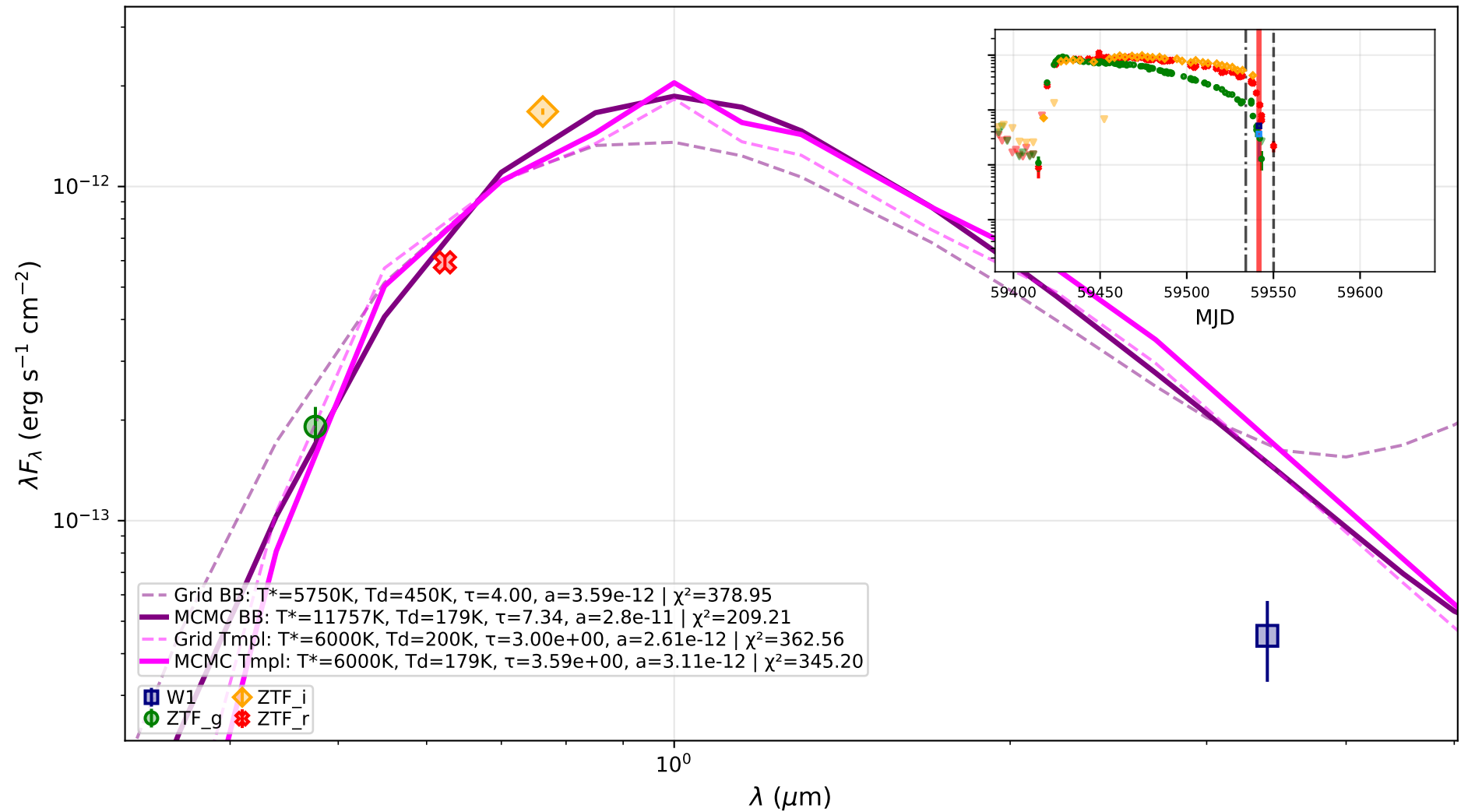
ZTF21abnlhxs: SED at MJD 59541.66 (Phase 123.7 d)
