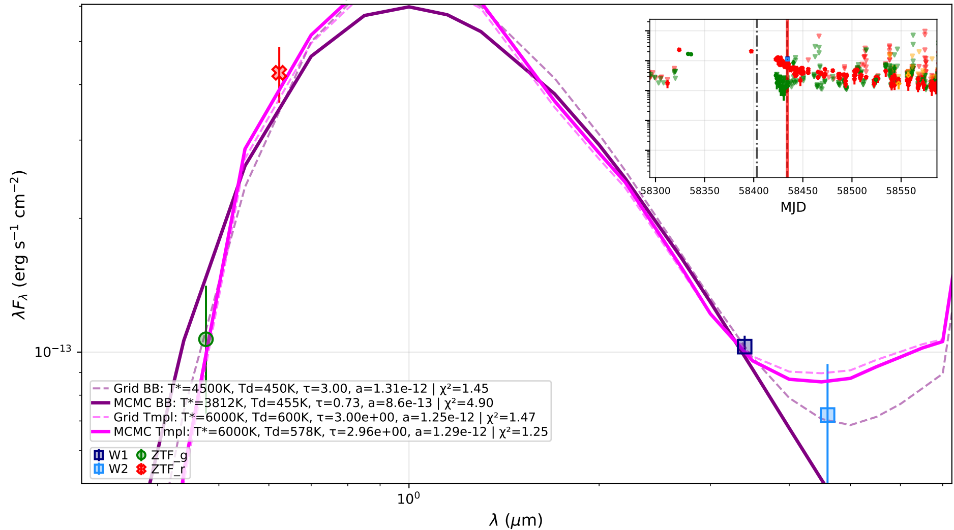
ZTF18abjndhh: SED at MJD 58434.36 (Phase 107.7 d)
