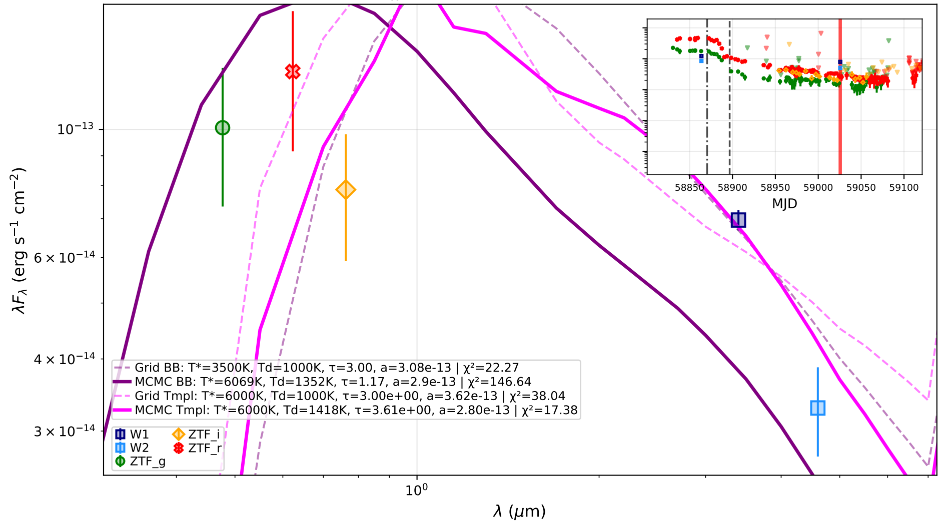
ZTF19acbwejj: SED at MJD 59025.65 (Phase 273.5 d)
