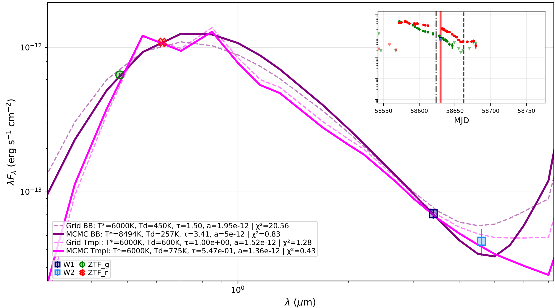
ZTF19aanrrqu: SED at MJD 58629.83 (Phase 60.0 d)
