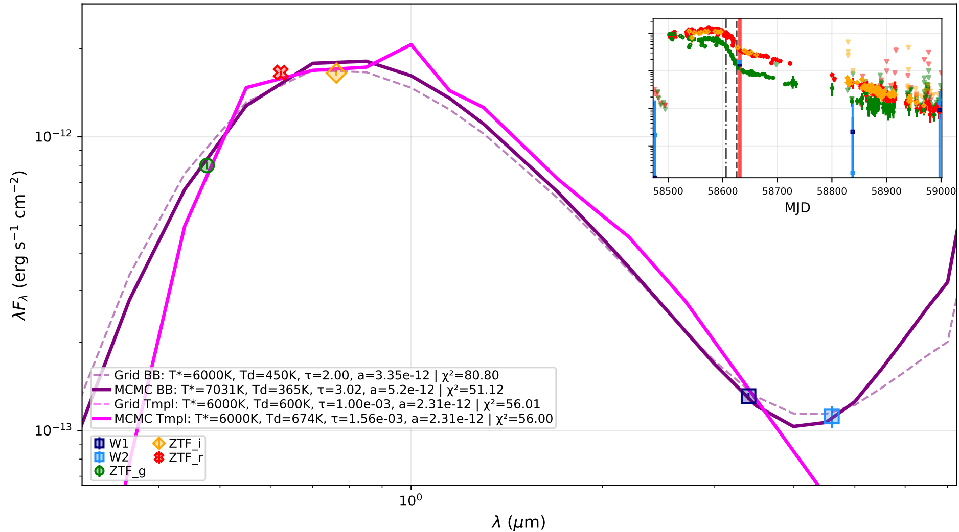
ZTF19aadnxxnl: SED at MJD 58631.44 (Phase 132.9 d)
