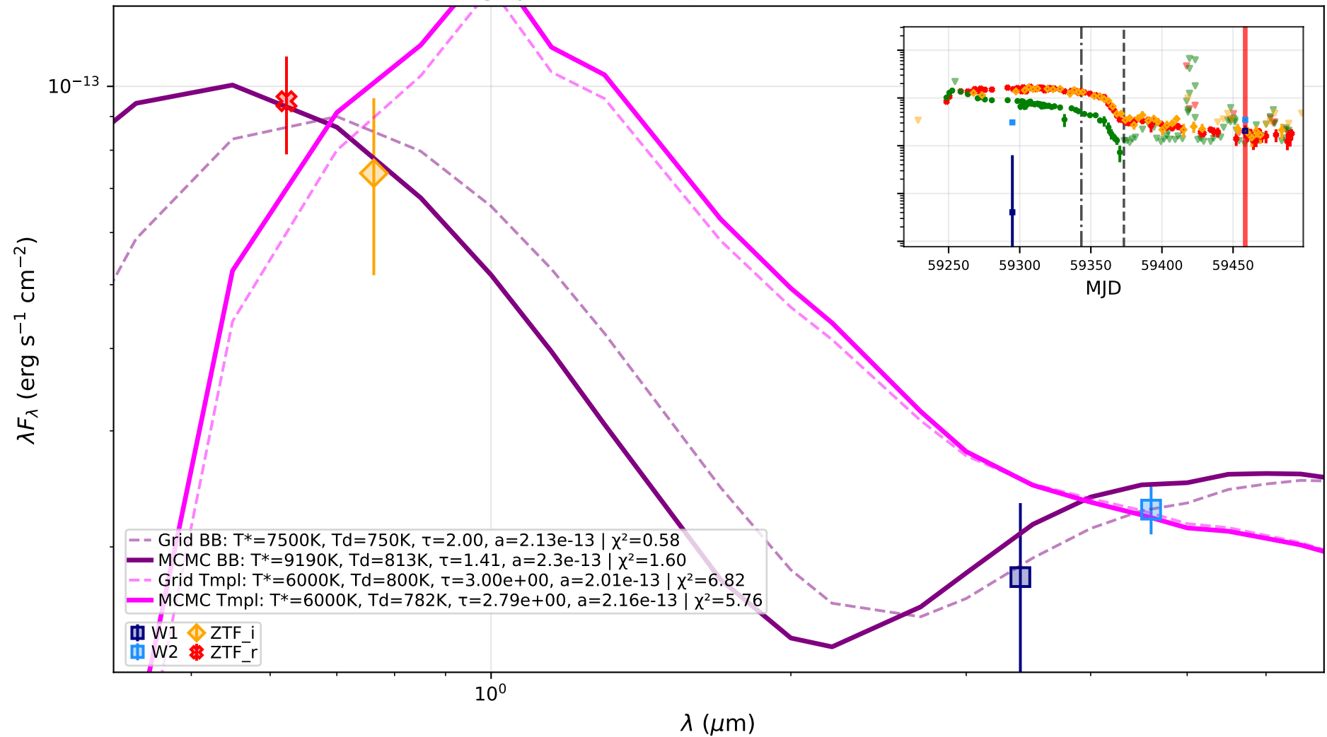
ZTF21aagtqna: SED at MJD 59458.55 (Phase 244.7 d)
