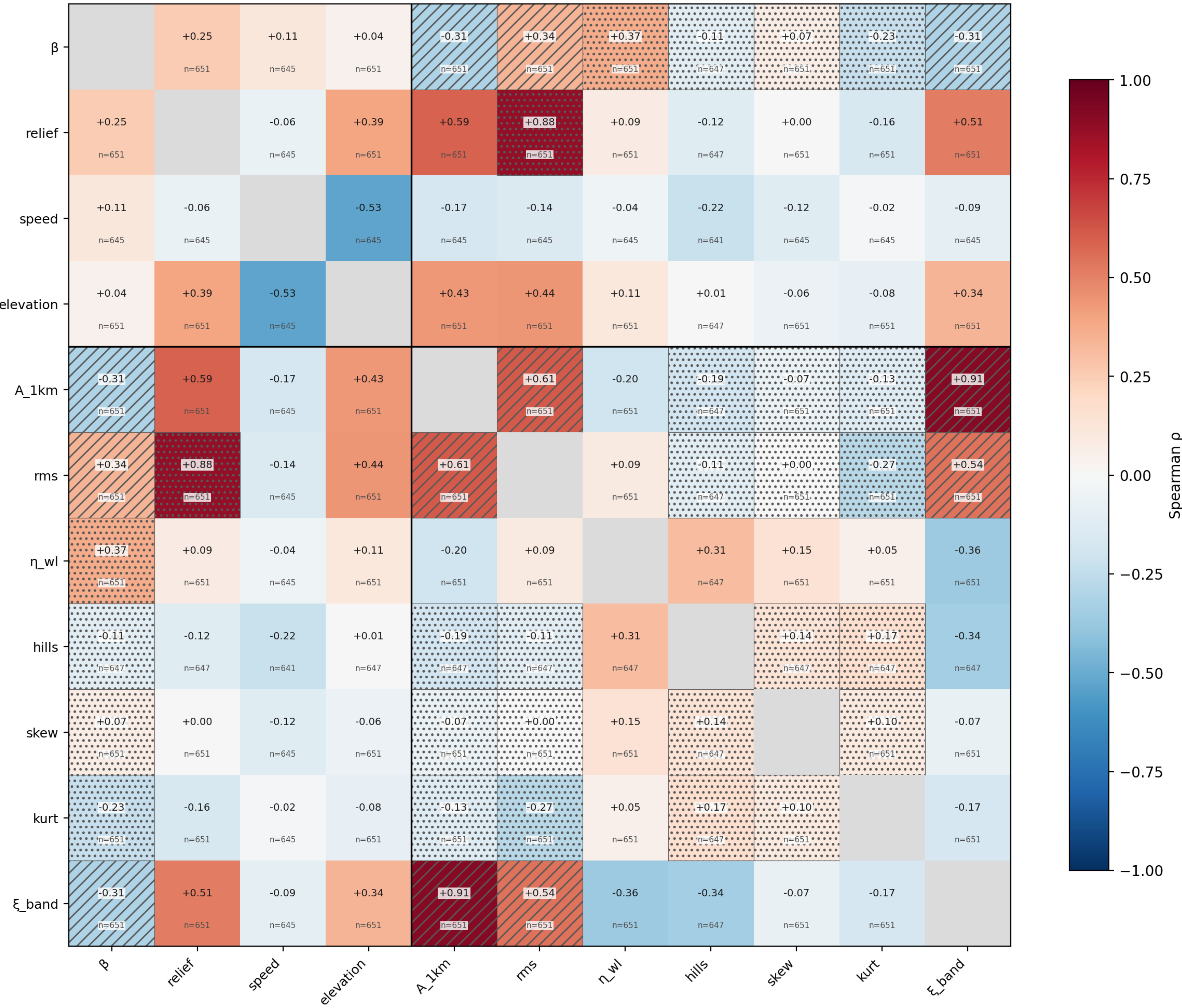
Vector element dependence — pooled (n per cell is pairwise-complete)
