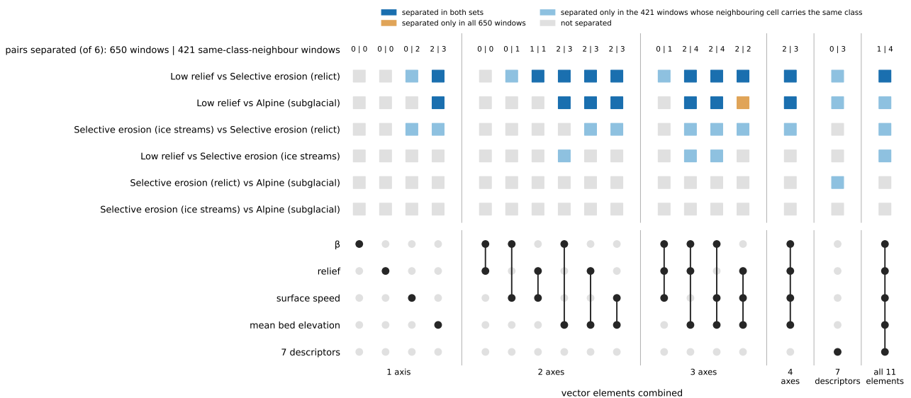
Figure 5.3: Separation of the Ockenden et al. [4] landscape classes by combinations of vector elements, over 650 analysed windows. Each column is one combination of the four classifying axes, the 7 descriptors together or all 11 elements together, and the black dots in the lower panel show the elements it uses. Square colour gives the two outcomes, and the numbers above each column are the counts of separated pairs in the two sets defined in the text (all 650 co-located windows, and the 421-window restricted set). Two classes are separated when the vector of their median differences is at least 1 pooled standard deviation long and at least a threshold number of standard errors long (depending on the number of elements in the combination), both measured with the covariance of the combined elements. Classes with fewer than 10 windows (Alpine (subaerial)) are not tested.
