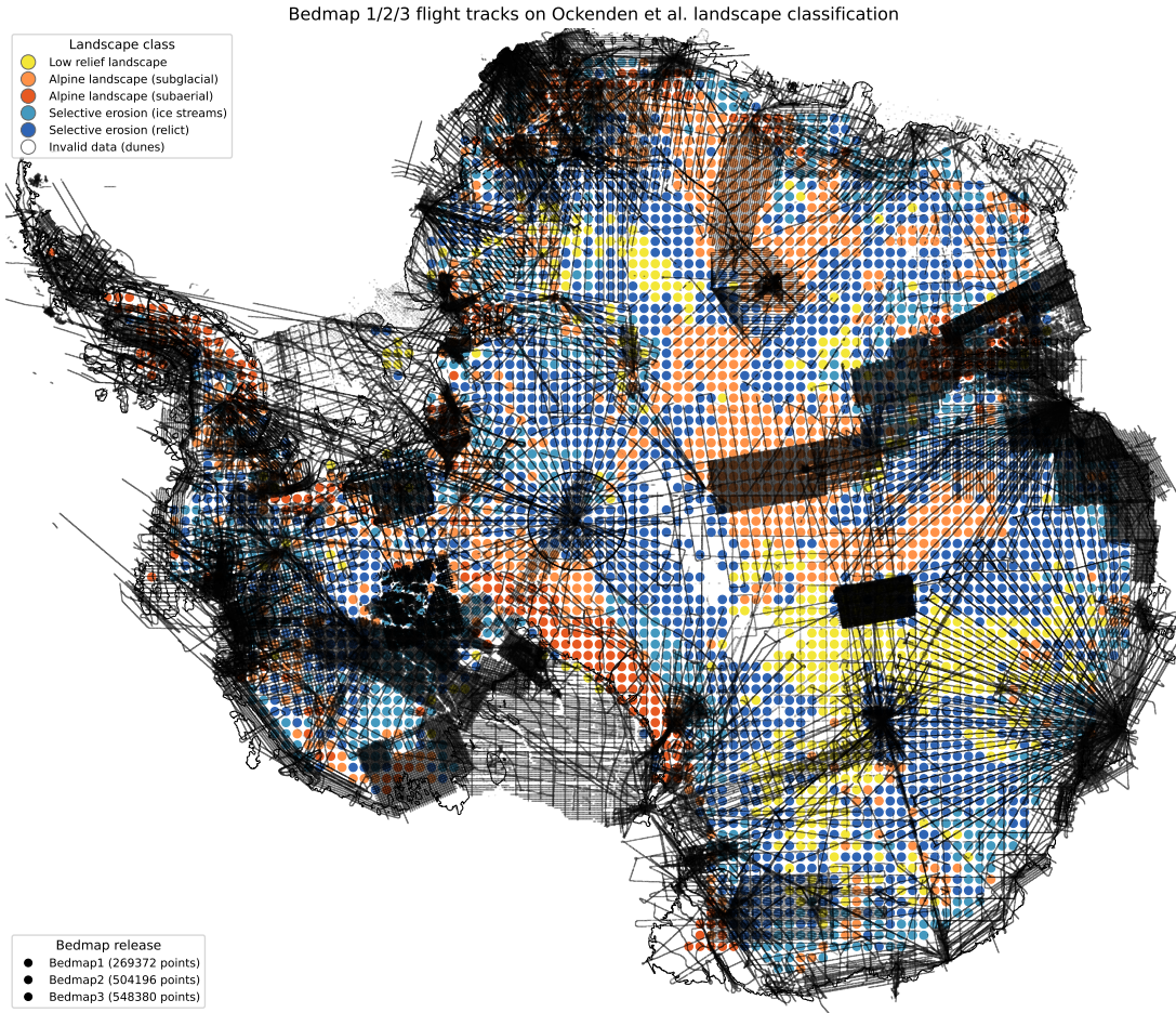
Figure 2.1: Bedmap1, Bedmap2 and Bedmap3 along-track survey points (black) over the continental landscape classification map by Ockenden et al. [4] (coloured cells, cells masked as invalid data (dunes) are drawn white). We reproduce the classification from the published metric grids [20] on 50 km cells. The point counts in the legend show the number of subsampled plotted points rather than published picks. ODSA operates on these along-track data, so the figure shows the sampling available to us across a continental landscape classification.
