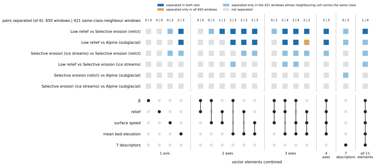
Figure 5.3: Separation of the Ockenden et al. [19] landscape classes by combinations of vector elements, over 650 analysed windows. Each column is one combination of the four classifying axes, the 7 descriptors together or all 11 elements together, and the black dots in the lower panel show the elements it uses. Square colour gives the two outcomes, and the numbers above each column are the counts of separated pairs in the two sets defined in the text (all 650 co-located windows, and the 421-window restricted set). Two classes are separated when the vector of their median differences is at least 1 pooled standard deviation long and at least a threshold number of standard errors long (depending on the number of elements in the combination), both measured with the covariance of the combined elements. Classes with fewer than 10 windows (Alpine (subaerial)) are not tested.
