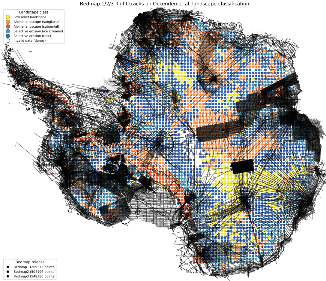
Figure 2.1: Bedmap1, Bedmap2 and Bedmap3 along-track survey points (black) over the continental landscape classification map by Ockenden et al. [19] (coloured cells, cells masked as invalid data (dunes) are drawn white). We reproduce the classification from the published metric grids [20] on 50 km cells. The point counts in the legend show the number of subsampled plotted points rather than published picks. ODSA operates on these along-track data, so the figure shows the sampling available to us across a continental landscape classification.
