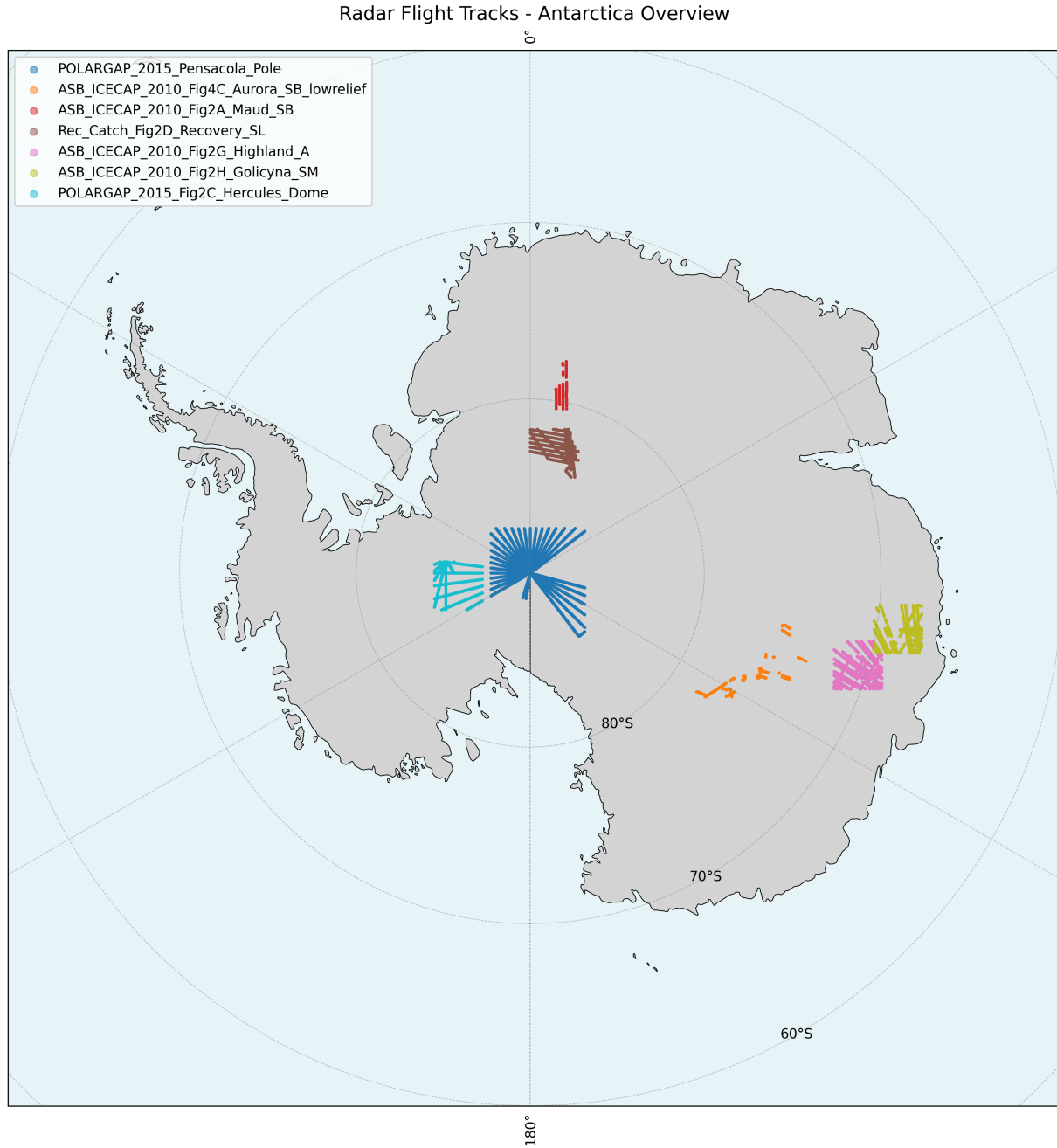
Figure 4.1: The seven RES survey regions we analysed with ODSA. Five regions use the PS71 boxes from [15]. The Aurora low-relief region is restricted to the low-relief cells of the Ockenden classification, and the Pensacola Pole Basin region uses a box that we defined.
