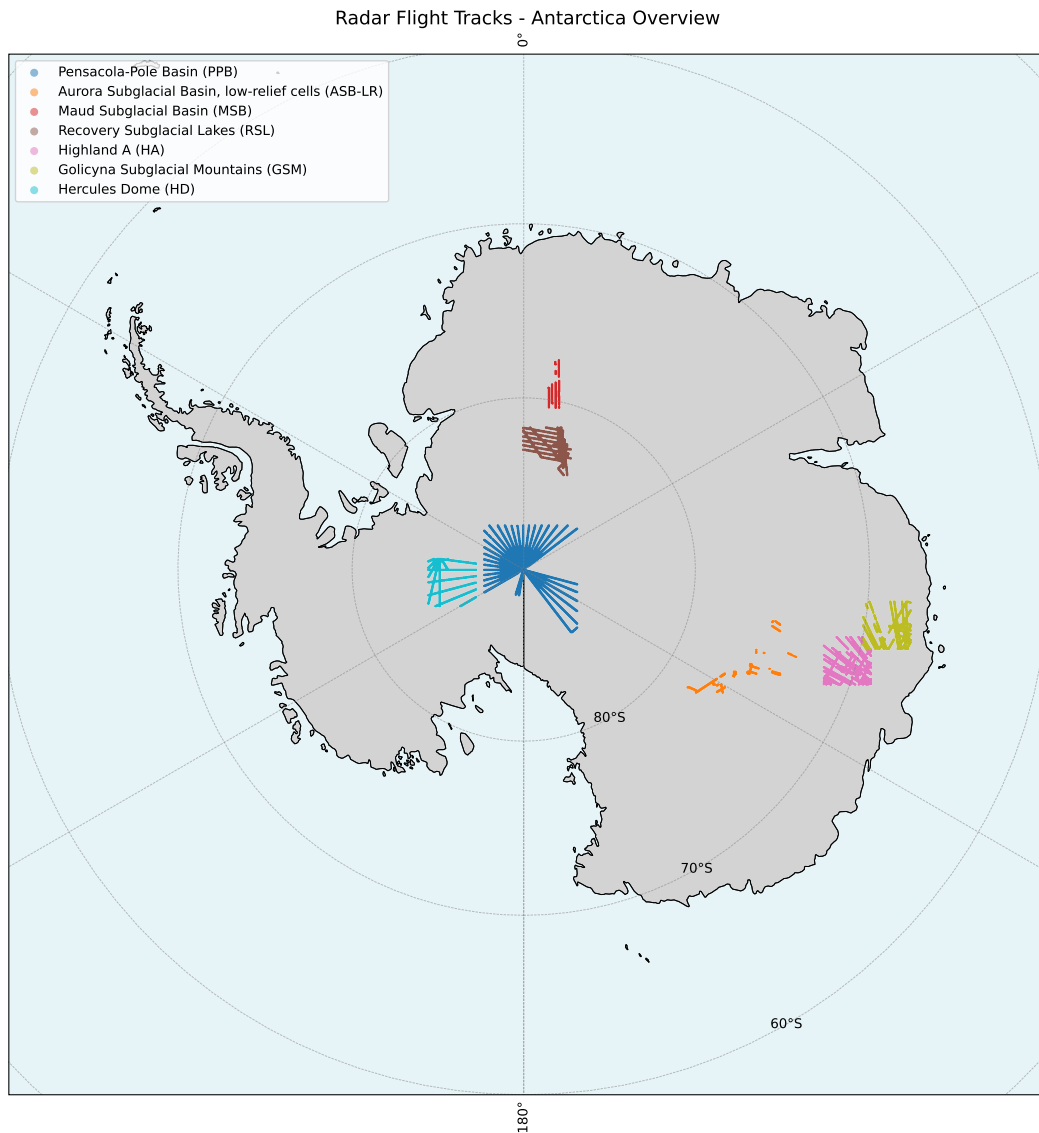
Figure 4.1: The seven RES survey regions analysed with ODSA. Five regions use the PS71 boxes from [20] directly, while the Pensacola Pole Basin region and the Aurora low-relief region use boxes that I defined, with the Aurora low-relief region restricted to cells selected as low-relief from the published metric grids of [20].
