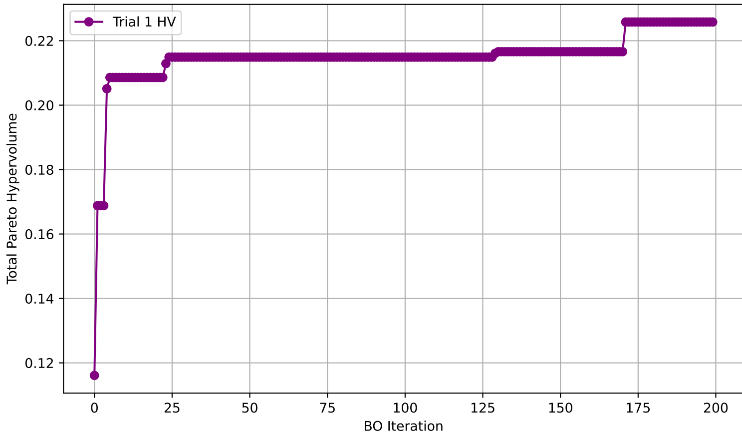
Pareto Hypervolume over BO Iterations for Perindopril MPO (Trial 1)
