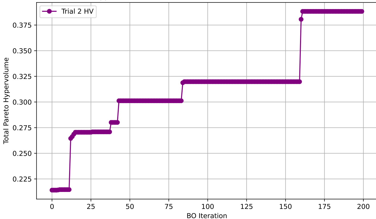
Pareto Hypervolume over BO Iterations for Fexofenadine MPO (Trial 2)
