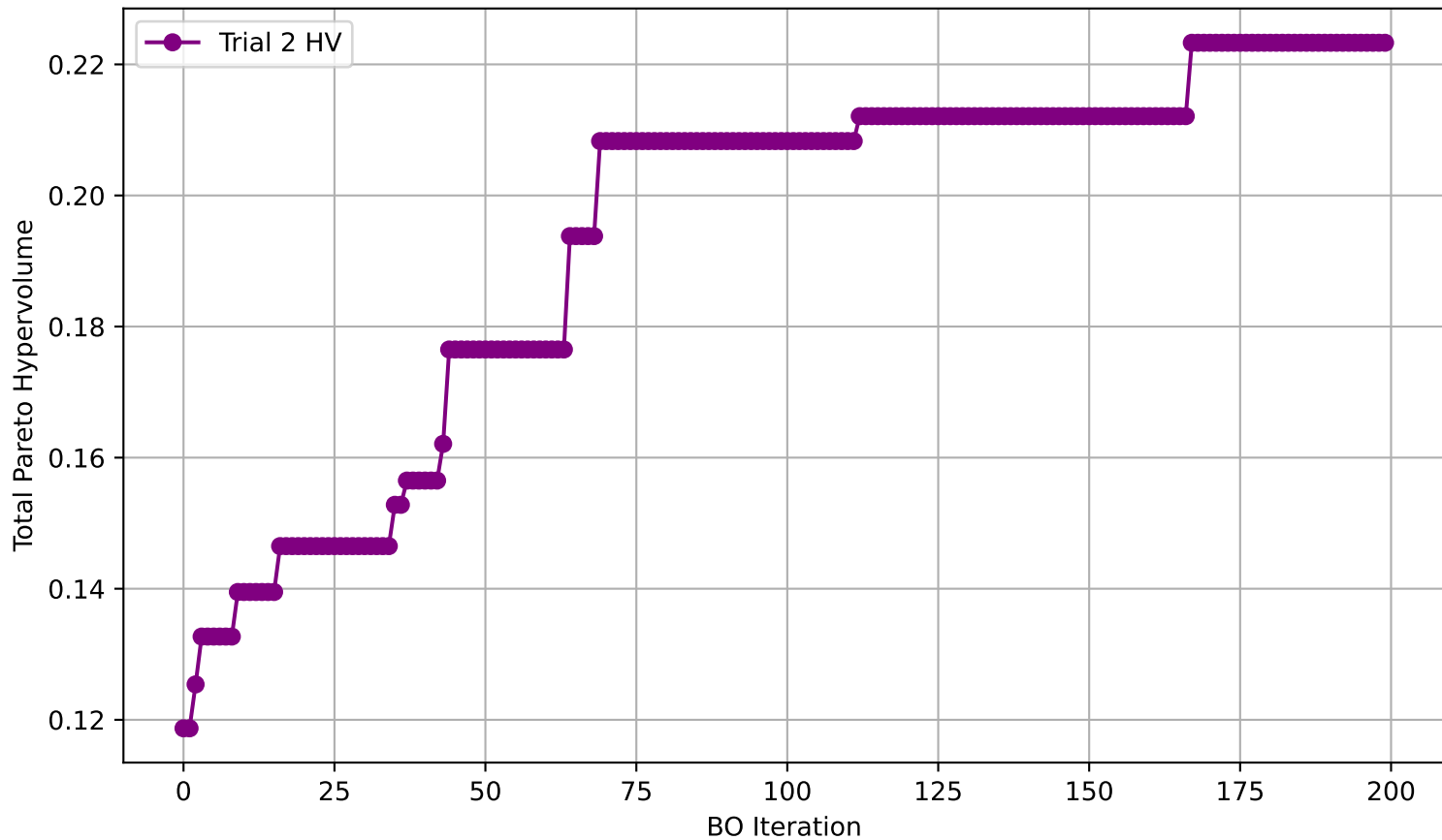
Pareto Hypervolume over BO Iterations for Perindopril MPO (Trial 2)
