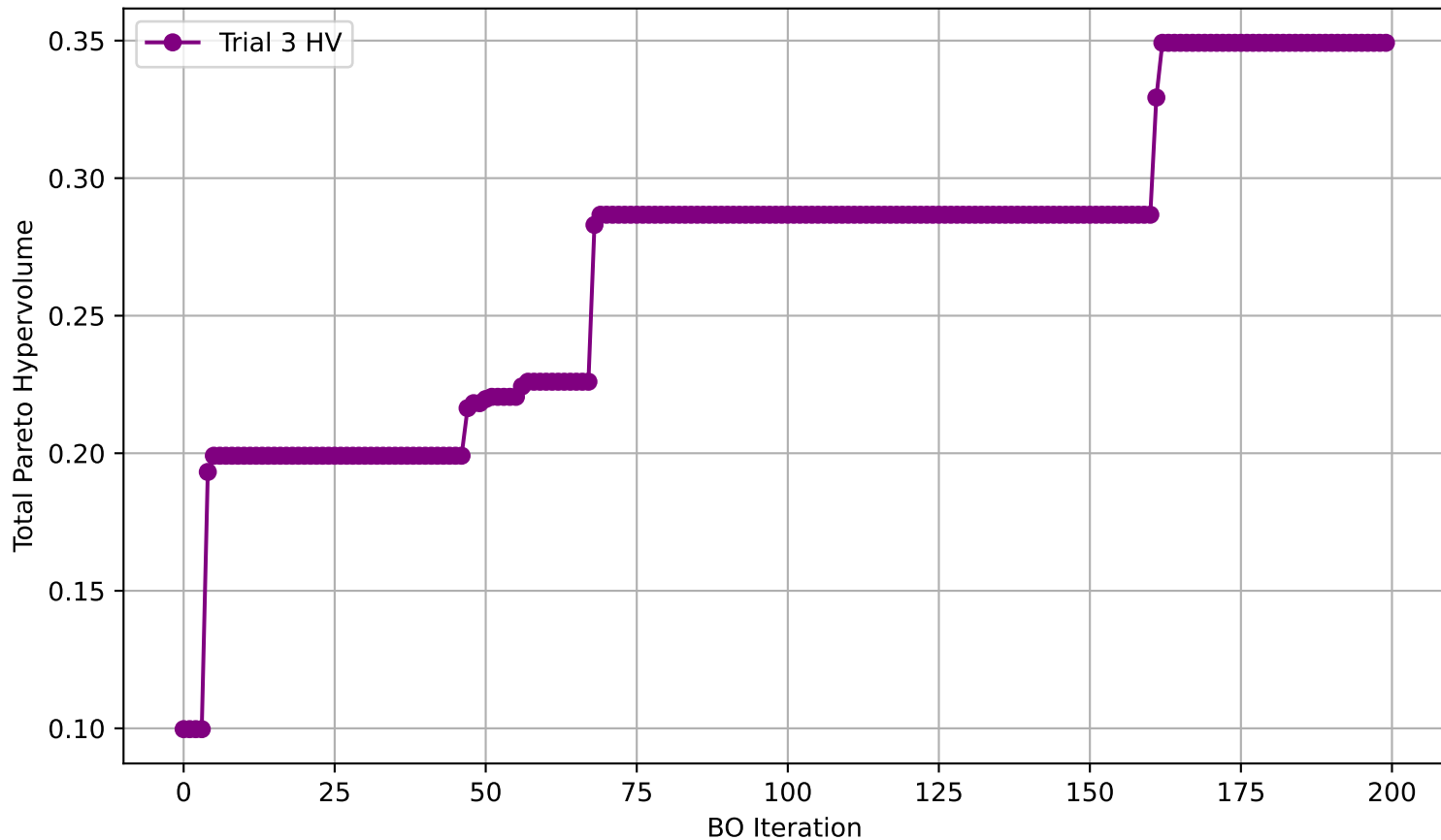
Pareto Hypervolume over BO Iterations for Amlodipine MPO (Trial 3)
