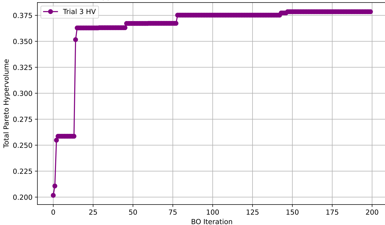
Pareto Hypervolume over BO Iterations for Fexofenadine MPO (Trial 3)
