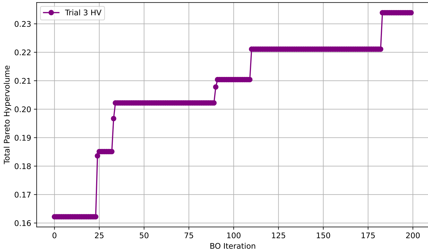
Pareto Hypervolume over BO Iterations for Perindopril MPO (Trial 3)
