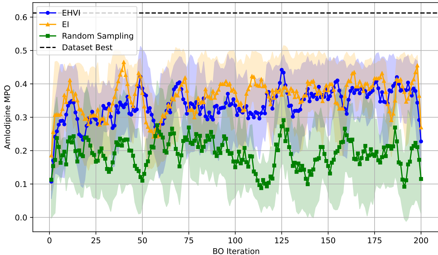
Amlodipine MPO (avg \pm std) over 3 Experiment Runs
