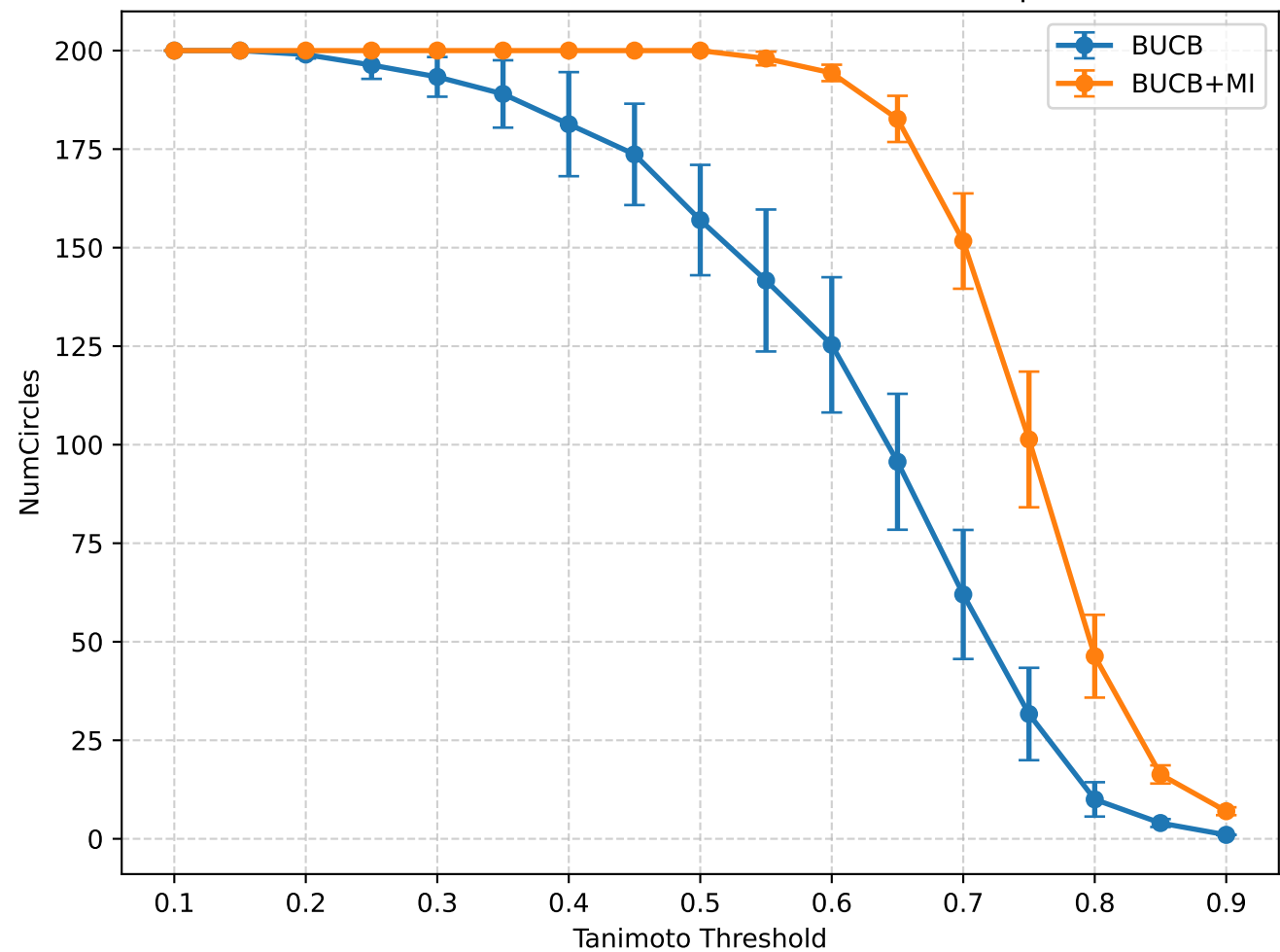
#Circles across thresholds (BUCB vs BUCB+MI, \beta=0.1 )
