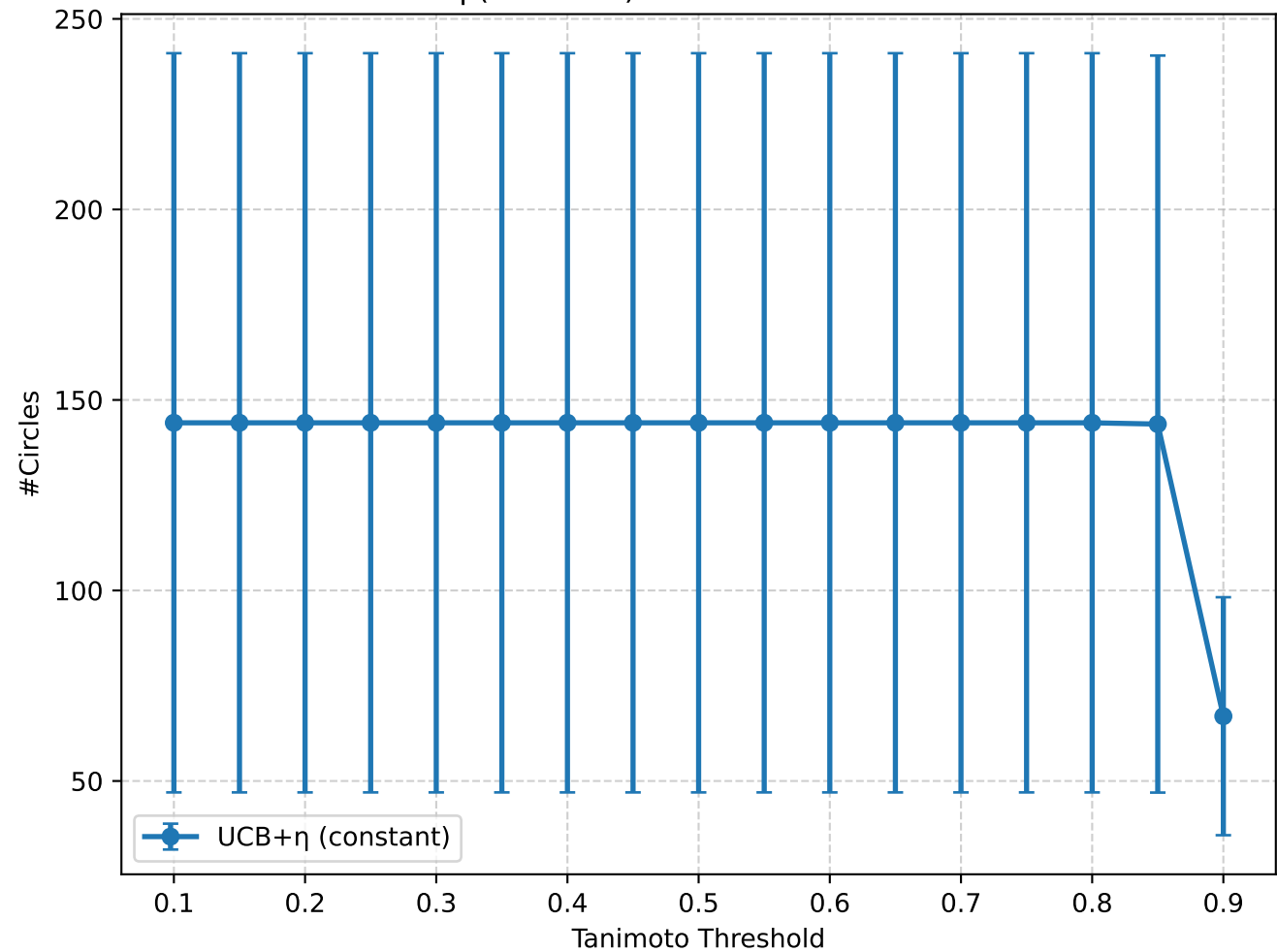
UCB+ \eta (constant): Circles across thresholds
