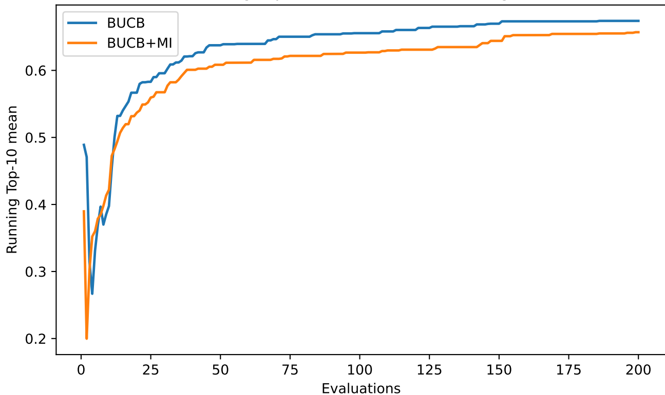
Running Top-10 vs. evaluations (averaged)
