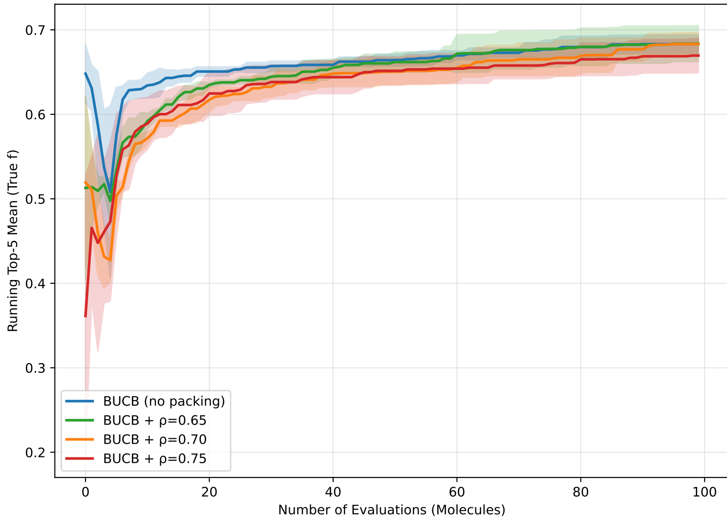
Top-5 Running Mean Curves — BUCB vs BUCB + \rho
