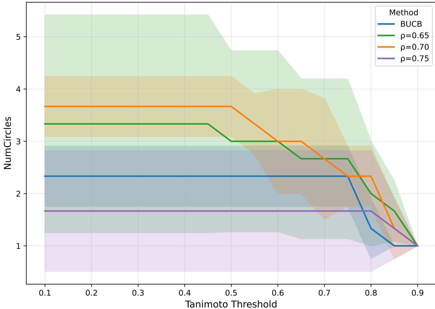
BUCB vs BUCB + Packing Constraint — #Circles Metric
