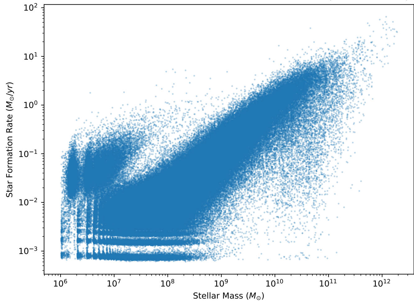
Stellar Mass vs. Star Formation Rate: EAGLE Simulation ( 0.0 < z < 0.5 )
