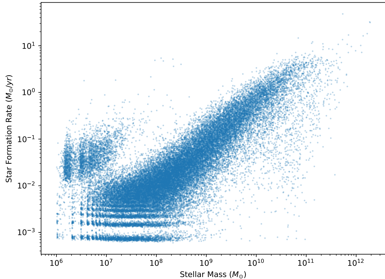
Stellar Mass vs. Star Formation Rate: EAGLE Simulation ( z = 0 )
