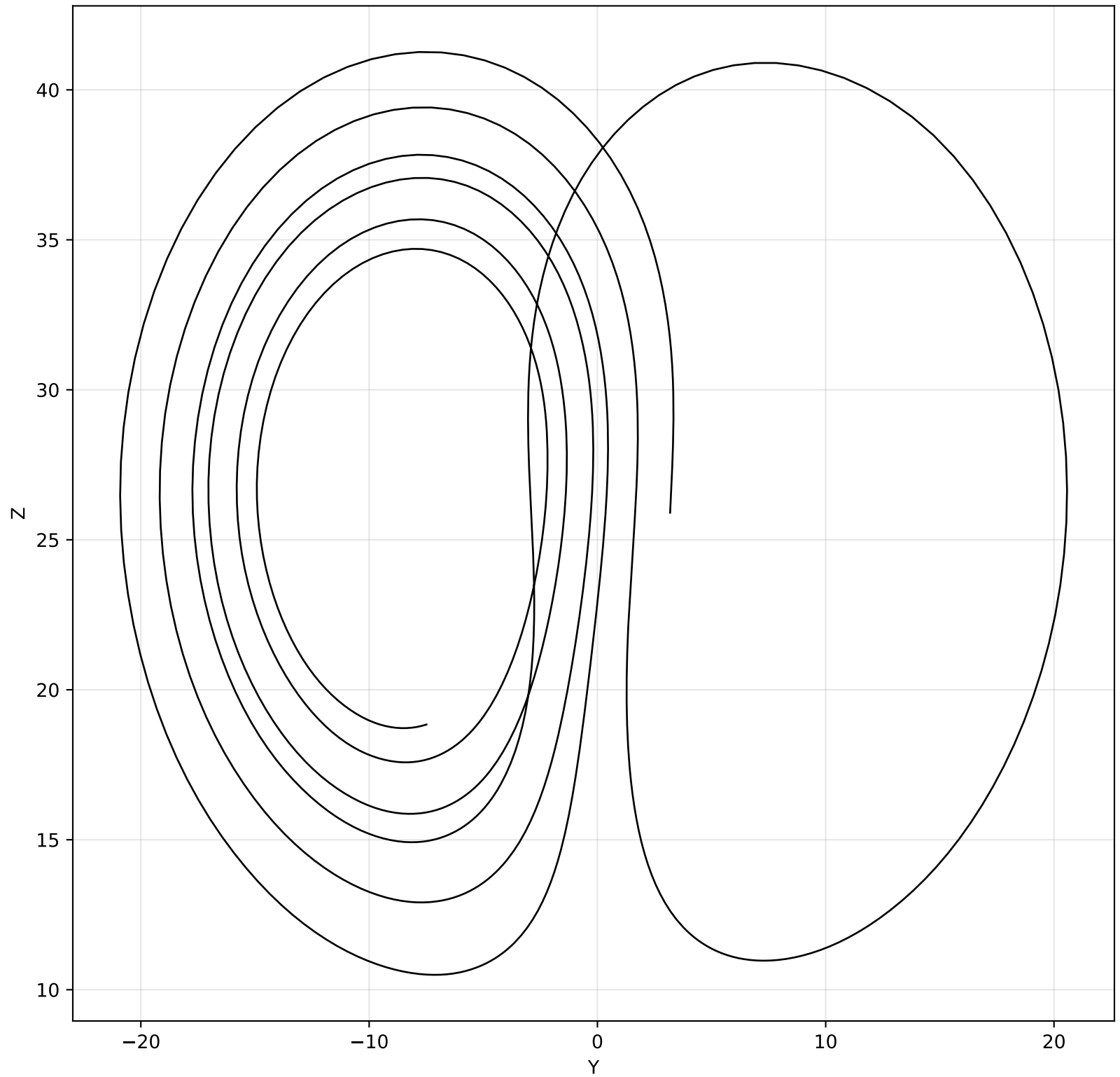
Lorenz Figure 2
