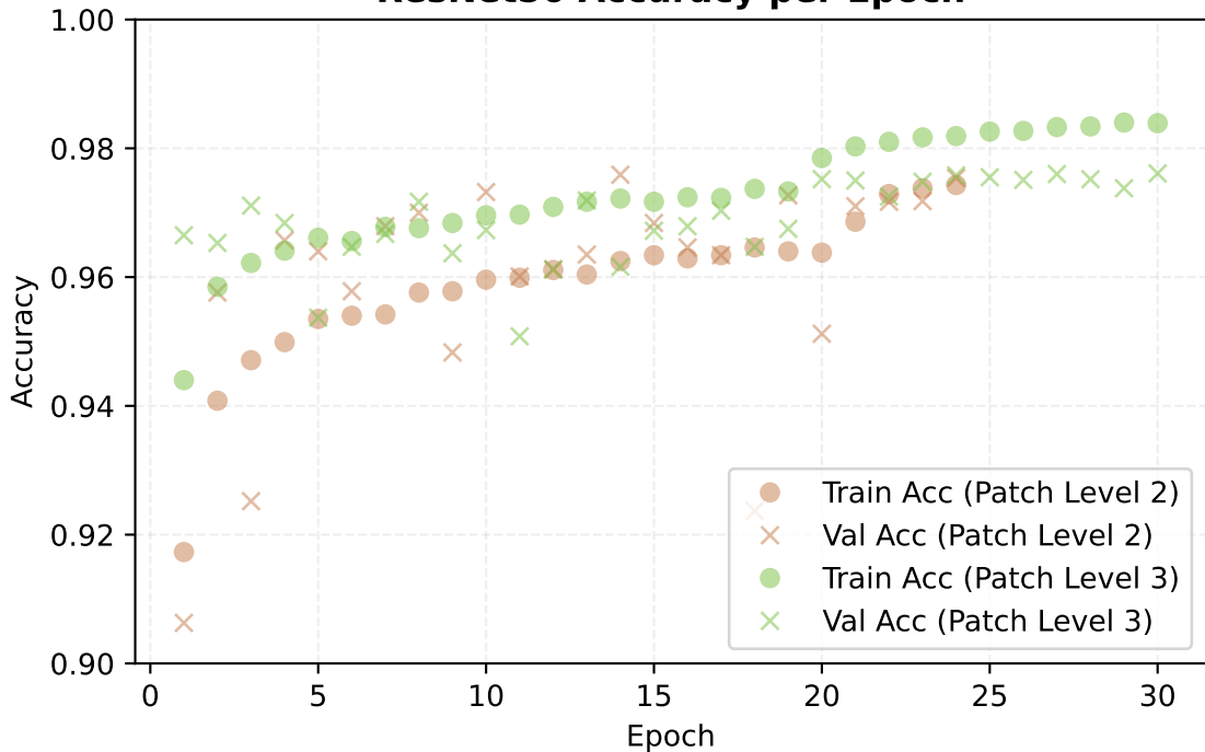
ResNet50 Accuracy per Epoch
