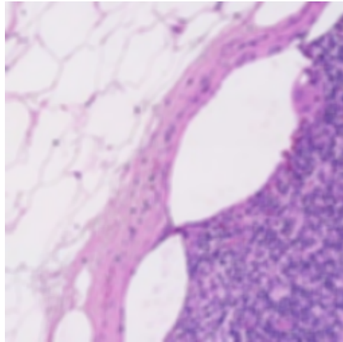
Gaussian Blur
