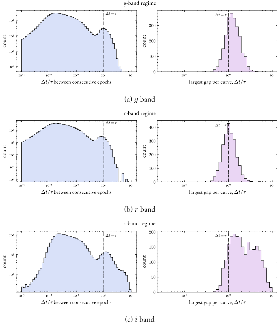
Figure 5.11: The spacing between consecutive epochs (left) and the single largest gap per curve (right), in units of the damping timescale, for the ZTF-matched simulations in each band. The line marks \Delta t = \tau .
