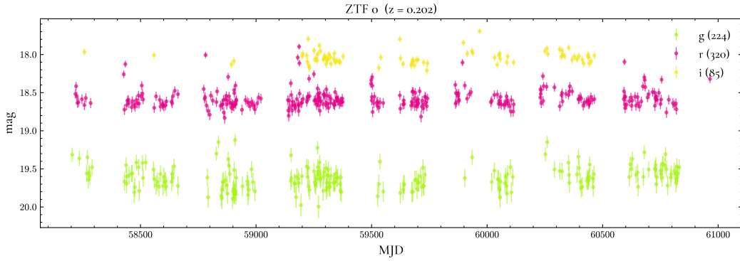
Figure 5.8: A real ZTF light curve of one AGN in the sample, showing the irregular cadence and seasonal gaps of a ground-based survey.
