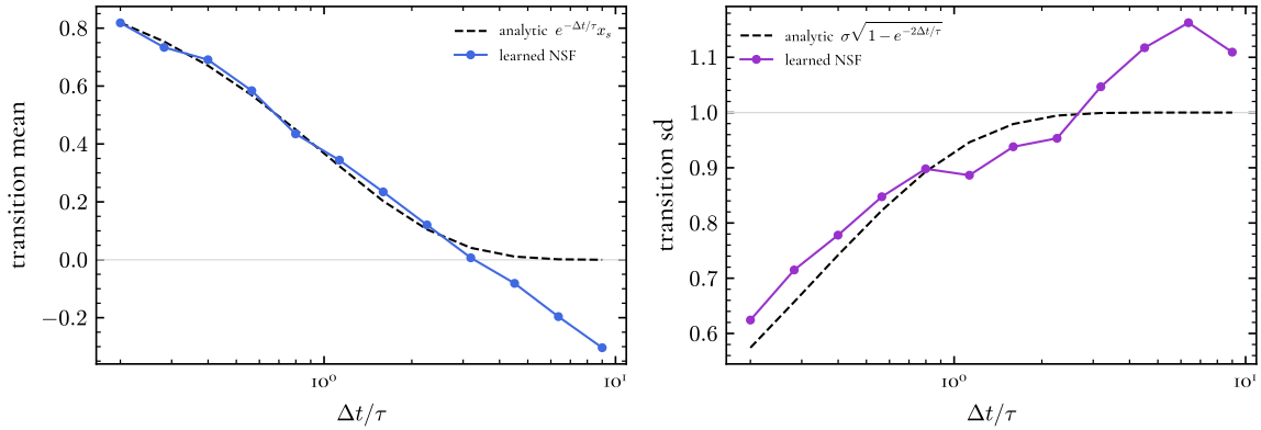
Figure 5.5: The mean (left) and standard deviation (right) of the learned transition, evaluated at the median damping timescale, compared with the analytic damped random walk (dashed). A small residual bias remains at the longest separations.
