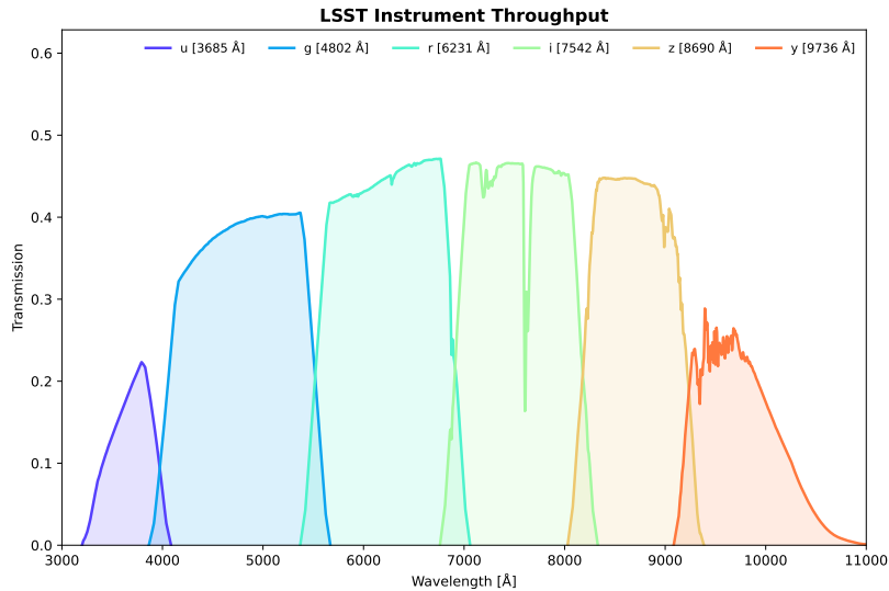
Figure 2.5: Total throughput of the six LSST bands u , g , r , i , z , and y , including atmospheric transmission, optics, and detector sensitivity.
