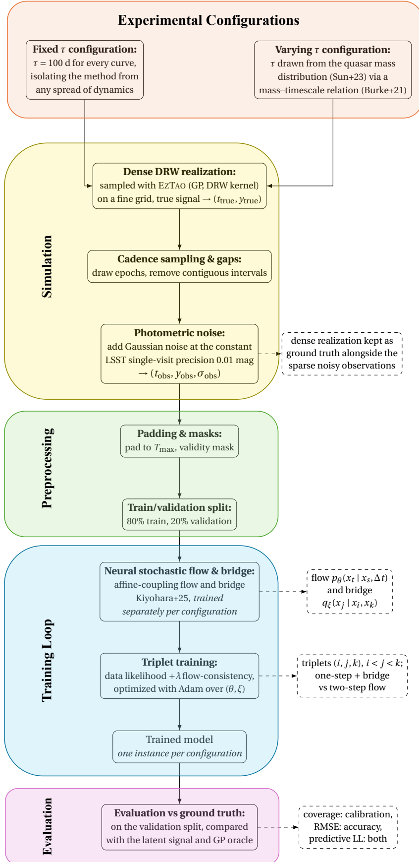
Figure 5.1: Pipeline of the idealized simulation experiments.
