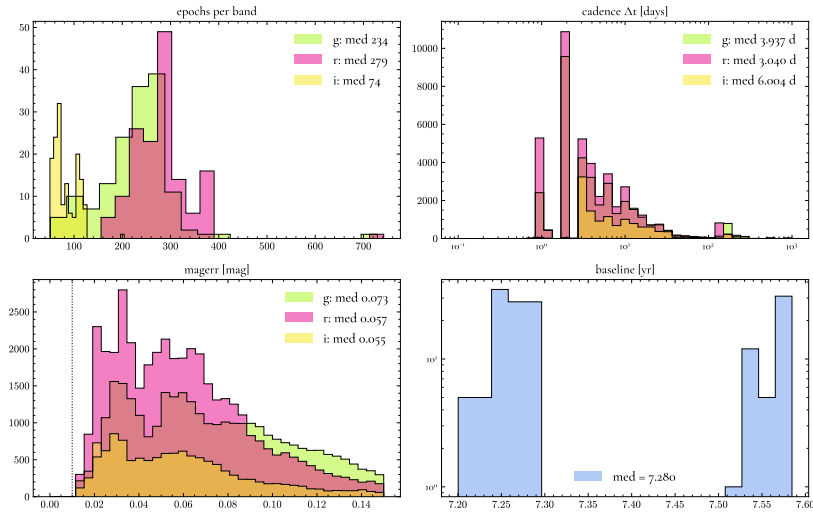
Figure 5.9: Distributions of the number of epochs, cadence, and photometric uncertainty across the 150 ZTF AGN in the g , r , and i bands.
