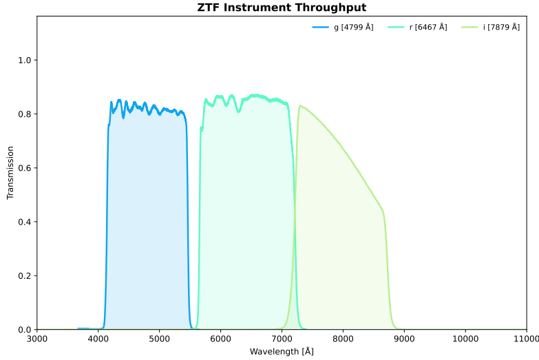
Figure 2.4: On-axis transmission of the three ZTF bands g , r , and i , with central wavelengths of 4799, 6467, and 7879 Å.
