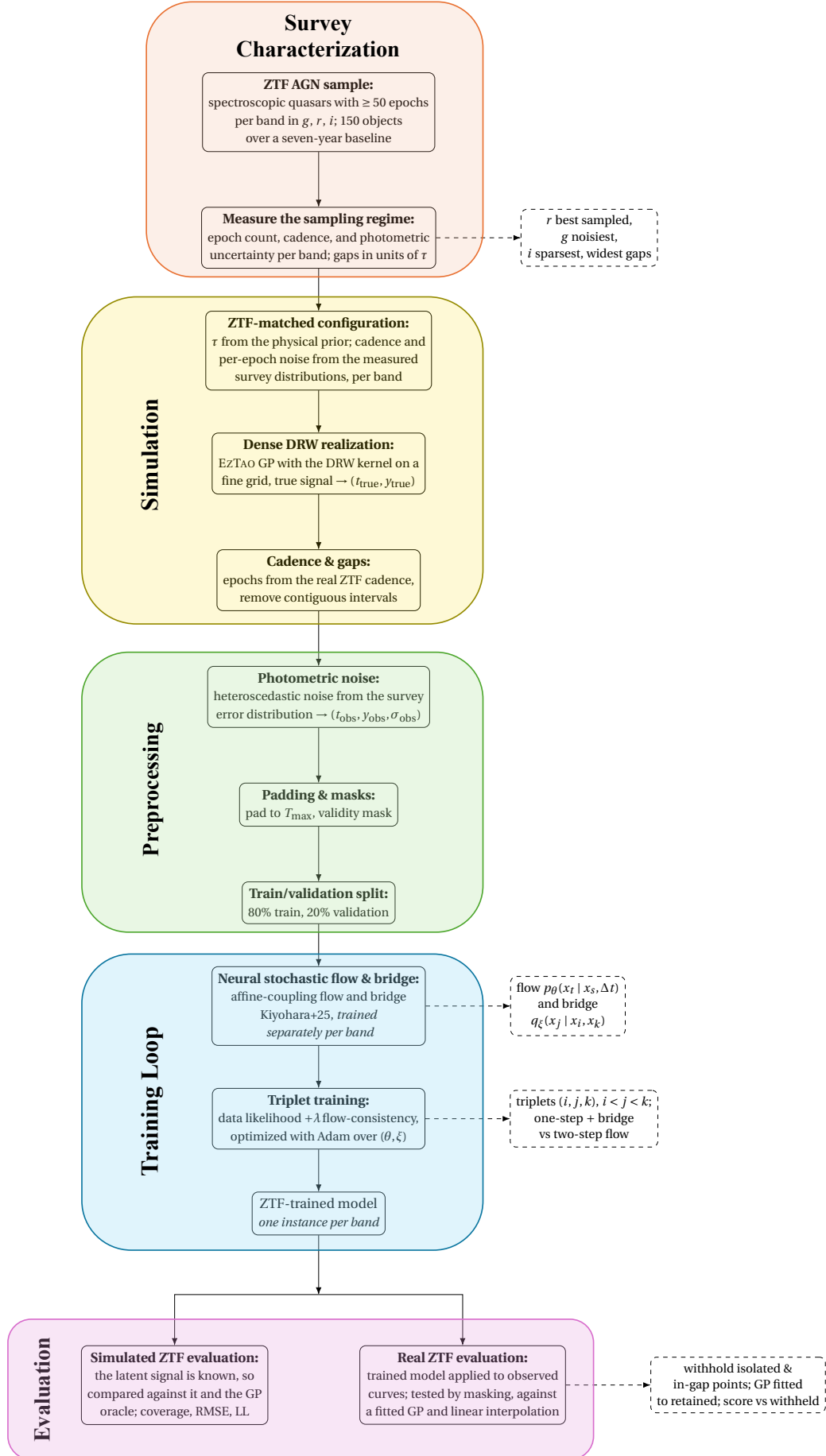
Figure 5.7: Pipeline of the ZTF experiments.
