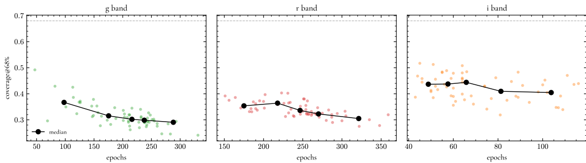
Figure 5.12: Coverage as a function of the number of epochs per curve, for the three ZTF bands where coverage worsens slightly as the number of epochs grows.
