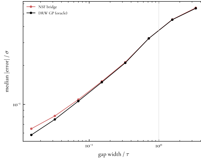
Figure 5.4: Reconstruction error as a function of gap width in units of the damping timescale, compared with the Gaussian process. The two track each other and converge at the widest gaps, where the correct prediction is the prior.
