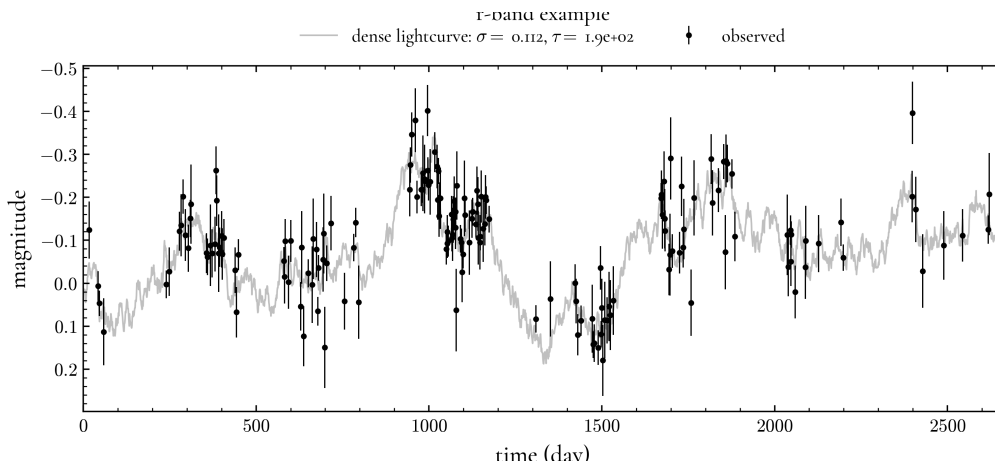
Figure 5.10: A simulated light curve from the ZTF-matched configuration, with the dense underlying realization and the sparse noisy observations drawn from it at the survey cadence.
