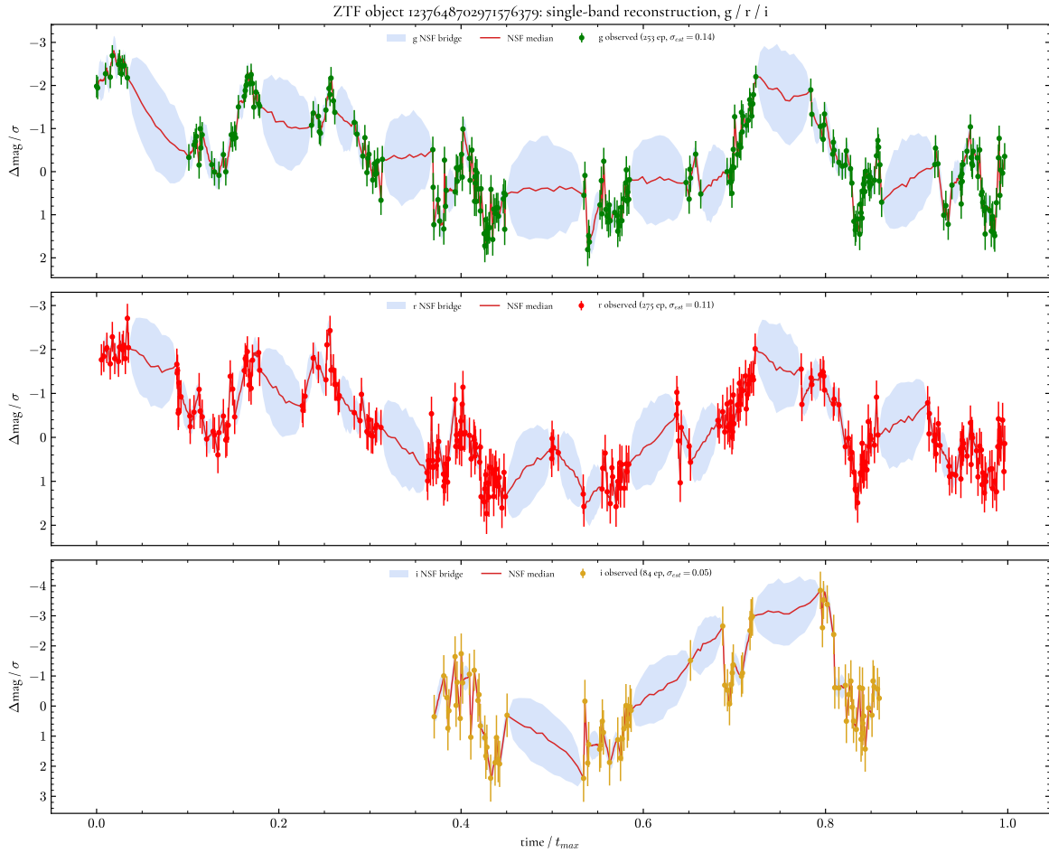
Figure 5.14: Reconstruction of a real ZTF light curve, showing the observations in green, red and yellow for the g , r , and i bands, respectively. The posterior median is shown in red, and the central 68% interval (shaded). The interval widens across the wider gaps in the real cadence.
