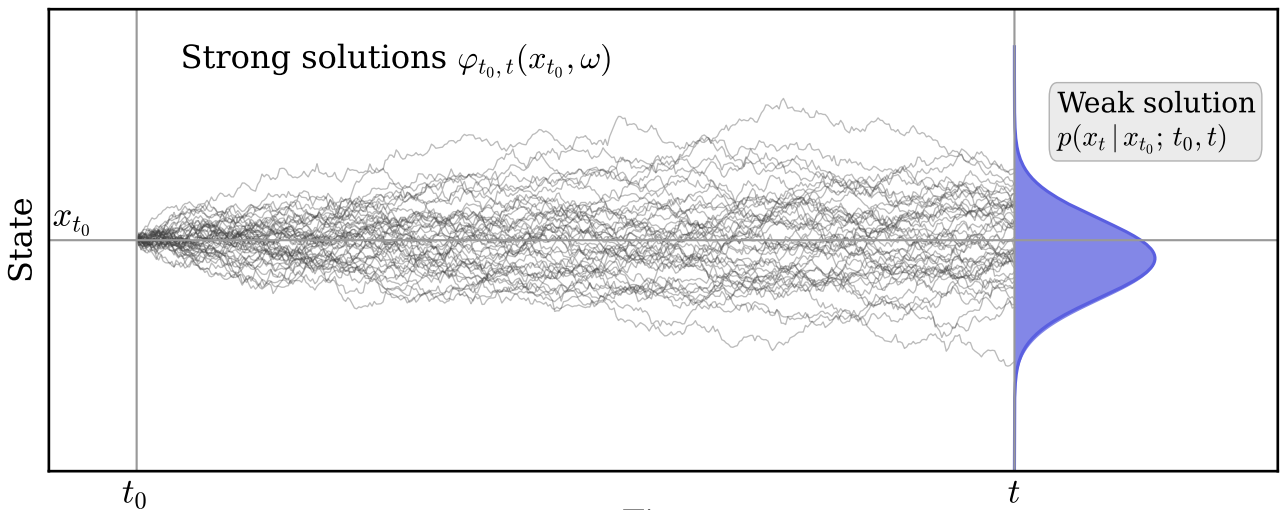
(a) Strong vs weak solution
