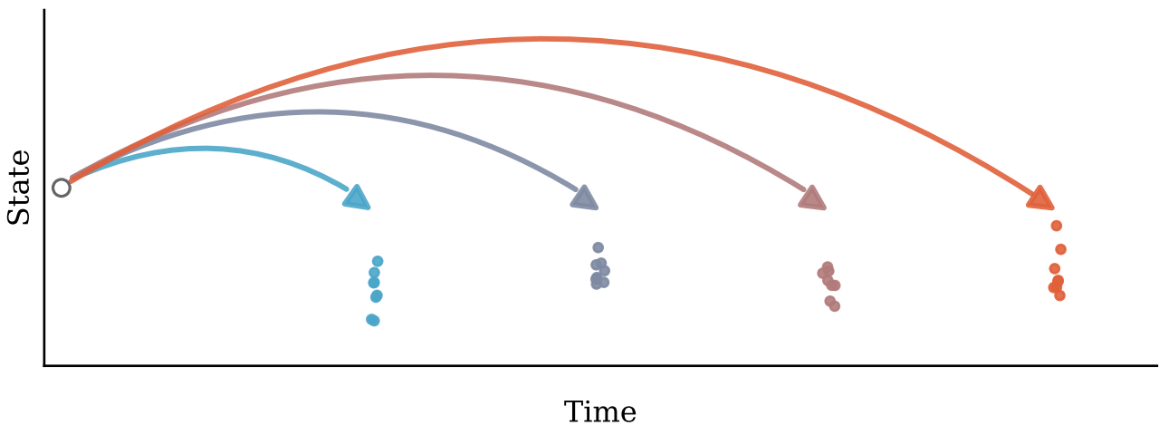
(a) Strong vs weak solution
