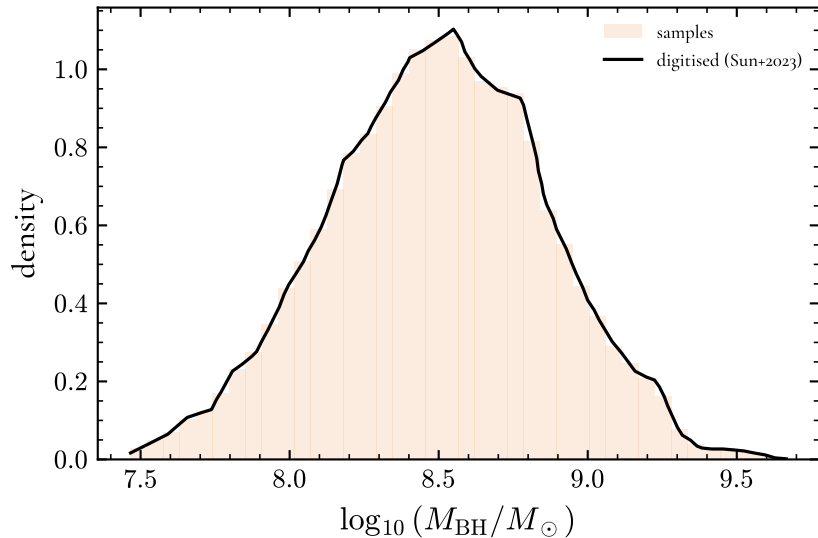
SMBH mass distribution
