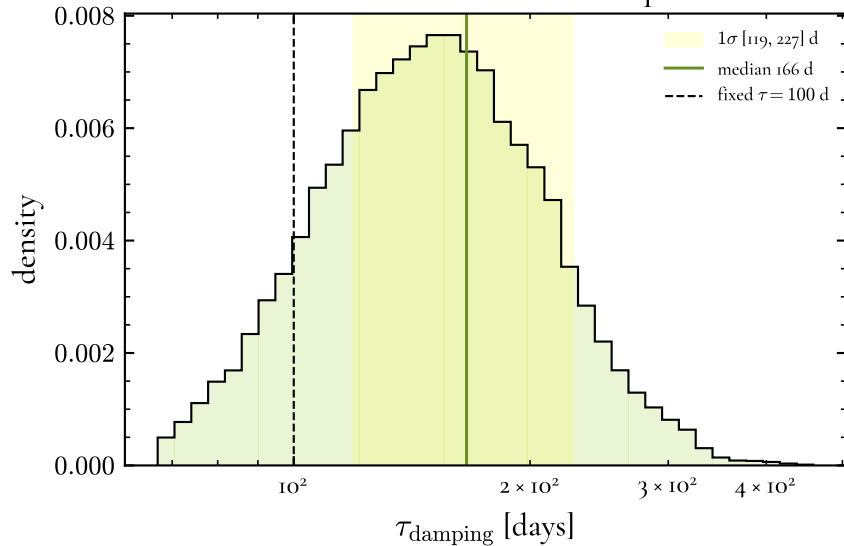
induced via Burke+2021 Eq. 1
