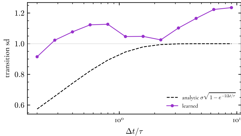
r-band, representative \tau = 166 d
