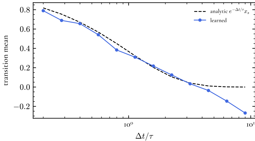
r-band, representative \tau = 166 d
