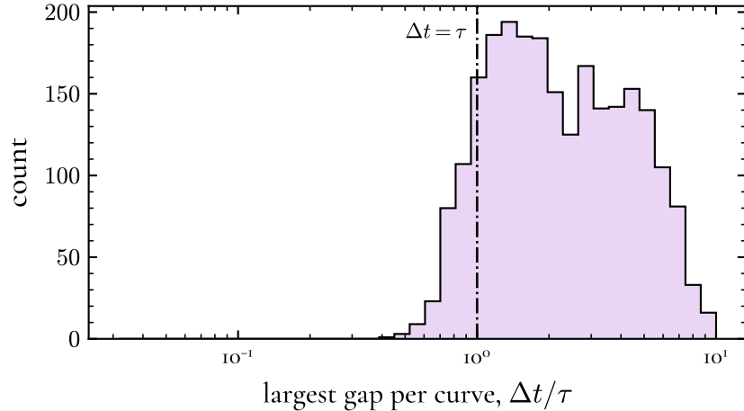
i-band regime
