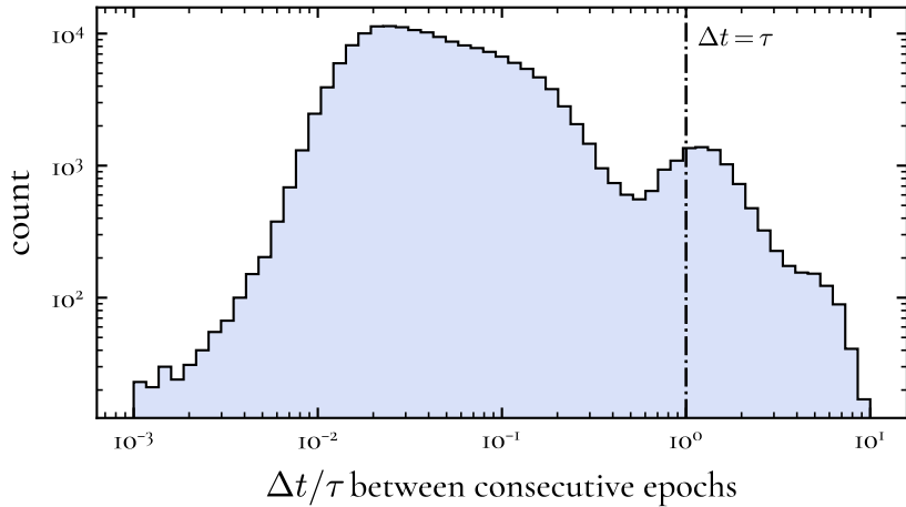
i-band regime
