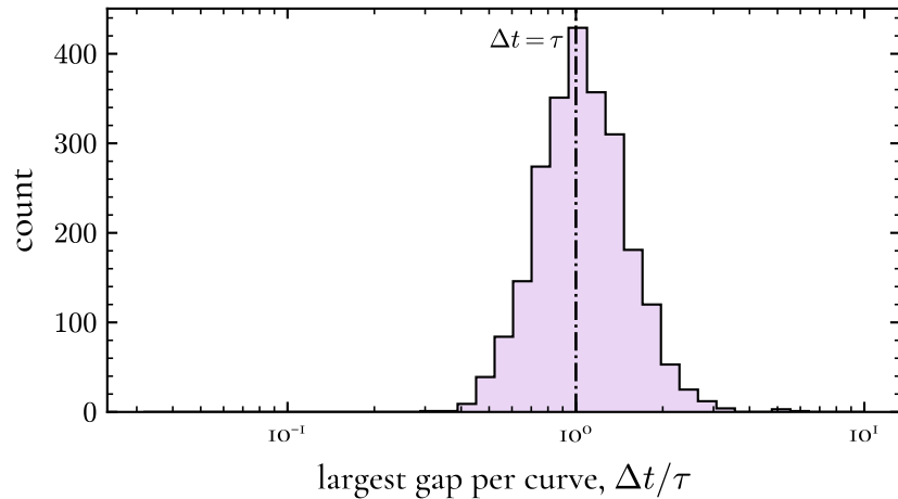
r-band regime
