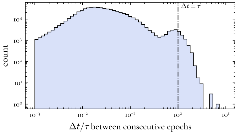
r-band regime
