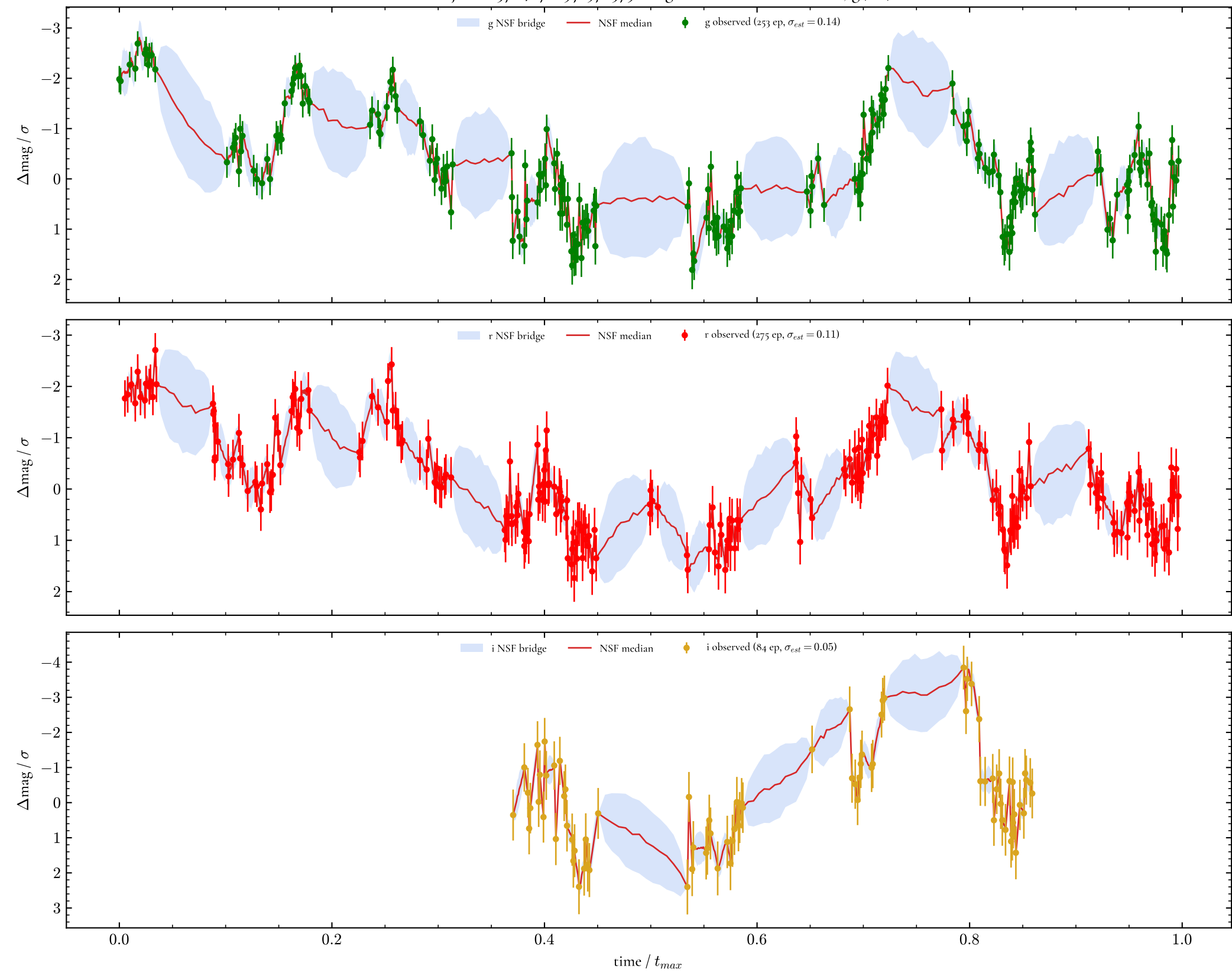
ZTF object 1237648702971576379: single-band reconstruction, g / r / i
