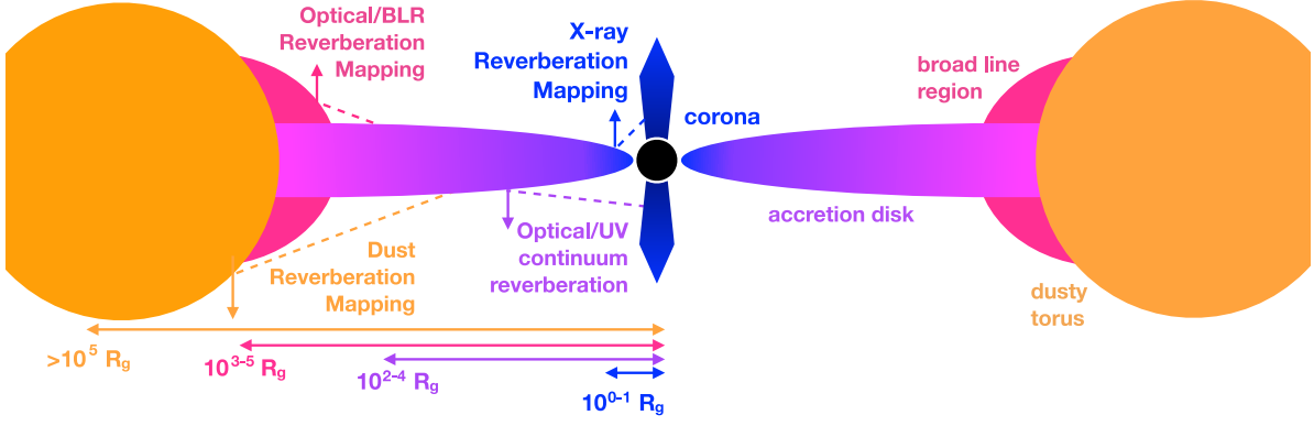
Figure 2.1: Cross-sectional schematic of an AGN illustrating the four main types of reverberation mapping and their corresponding radial scales from the central black hole. Taken from Cackett et al. 2021.
