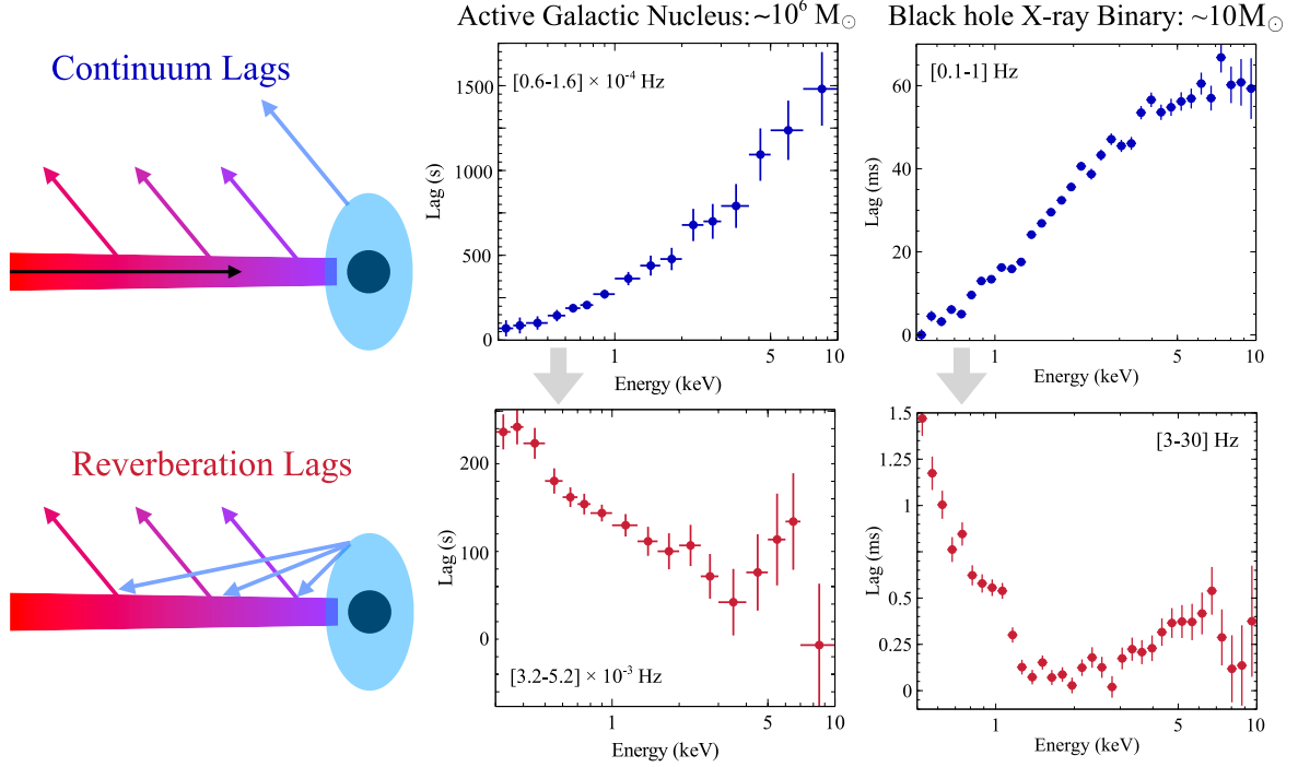
Figure 2.2: Frequency-resolved X-ray time lags as a function of energy for an AGN ( \sim 10^6 M_\odot , left) and a black hole X-ray binary ( \sim 10 M_\odot , right), illustrating the universality of the two lag regimes. At low Fourier frequencies (top, blue), hard X-rays lag soft ones, consistent with inward-propagating accretion fluctuations. At high Fourier frequencies (bottom, red), soft X-rays lag hard ones, consistent with disk reverberation. Taken from Kara and García 2025.
