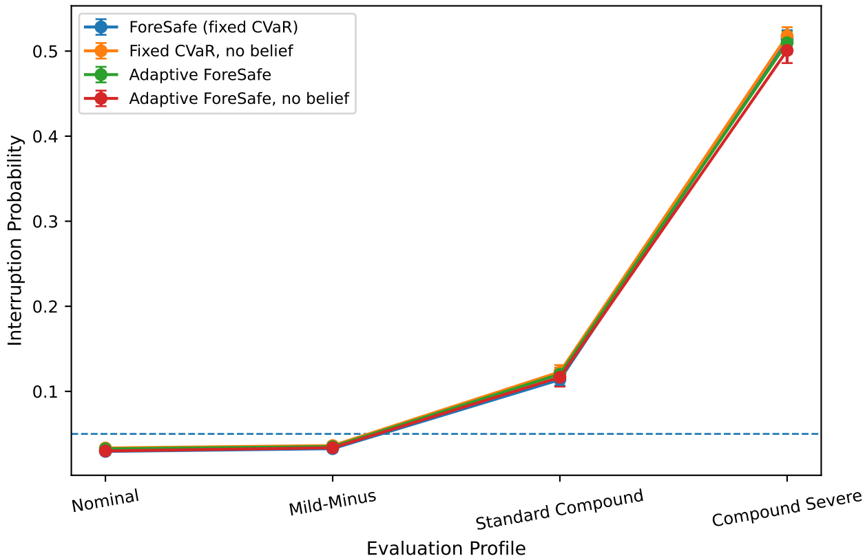
Ablation of Temporal Belief and Predictive Tightening
