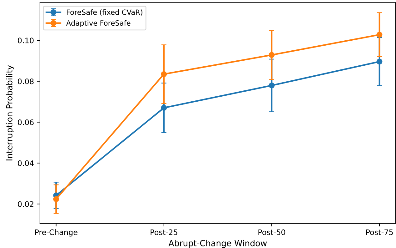
Response to Abrupt Channel/CSI Change
