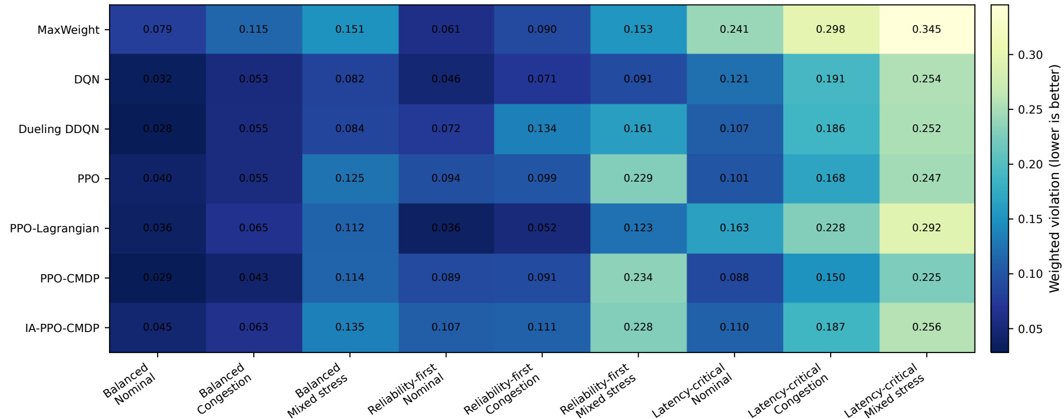
Context-wise weighted violation across matched static evaluation
