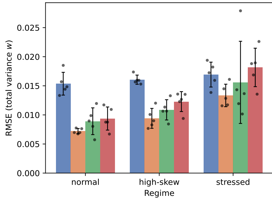
Held-out RMSE
