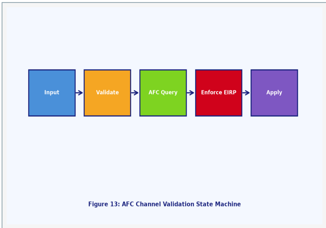
Figure 13 — AFC Channel Validation State Machine
